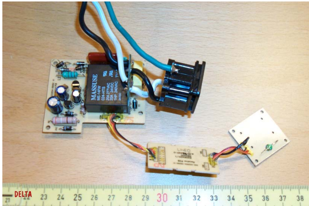
Photo 4 HA04. As photo 3 but with other side of prints turned up. RF module removed.
