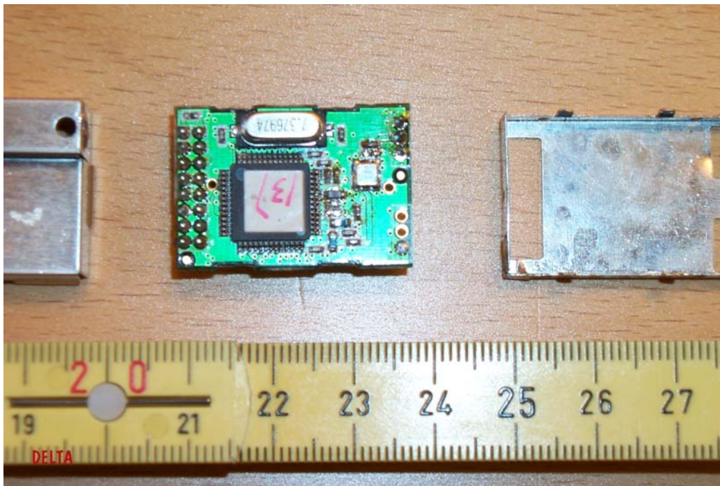
Photo 5 RF Module. Screens removed. ASIC side of module
