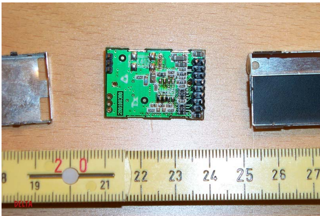
Photo 6 RF Module. Screens removed. ASIC side down.
