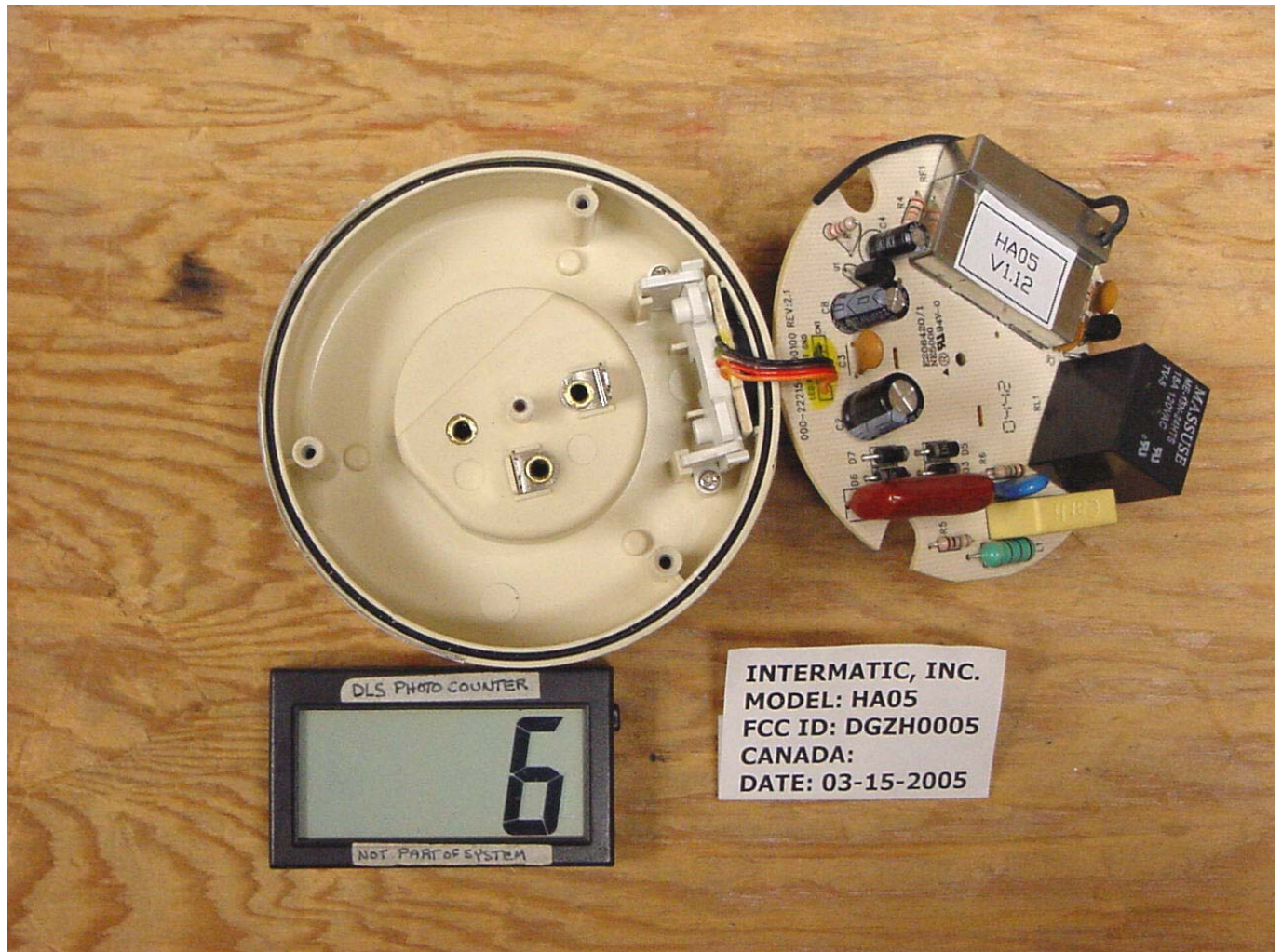
Circuit Board Removed
