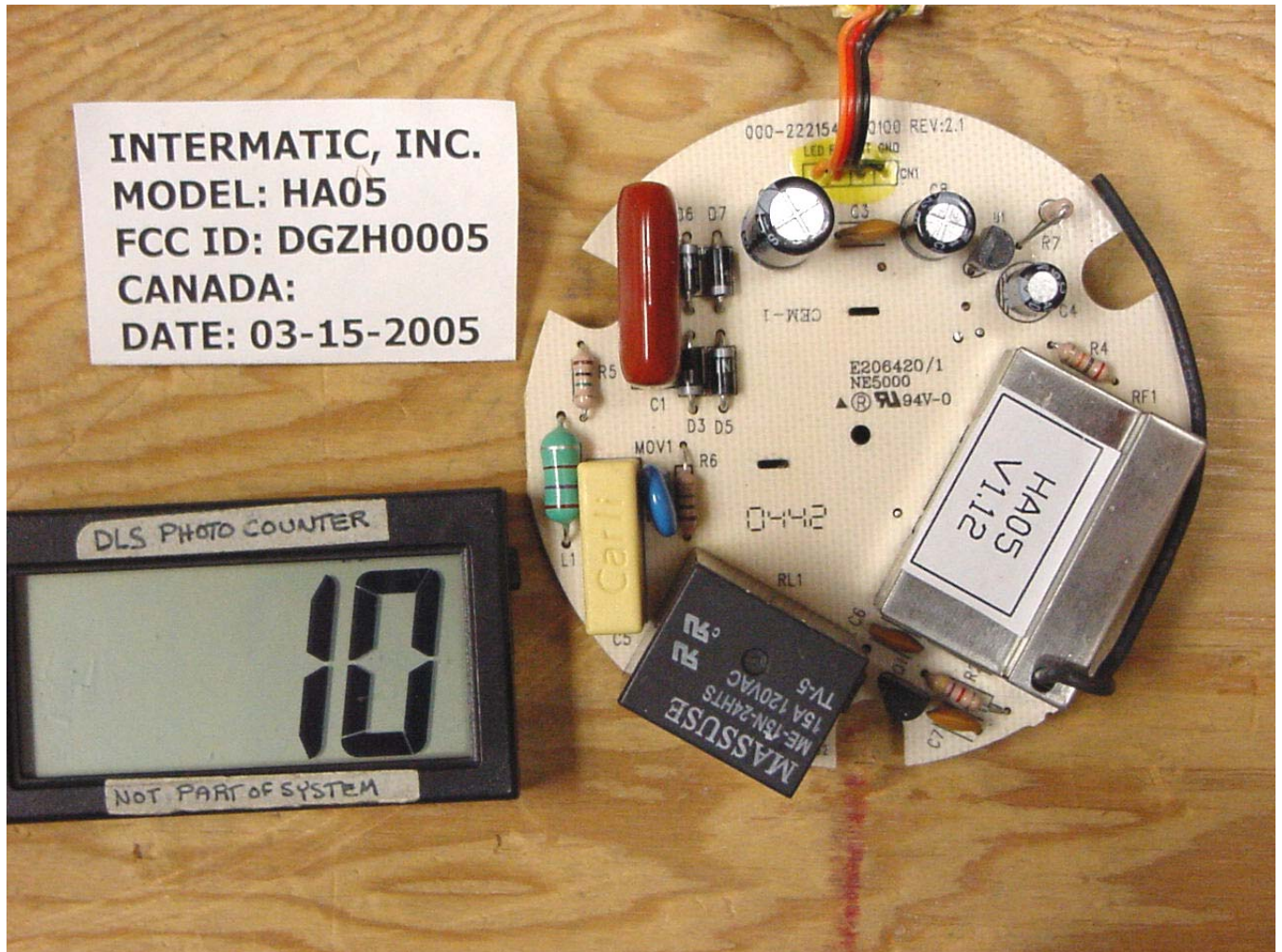
Circuit Board Component Side
