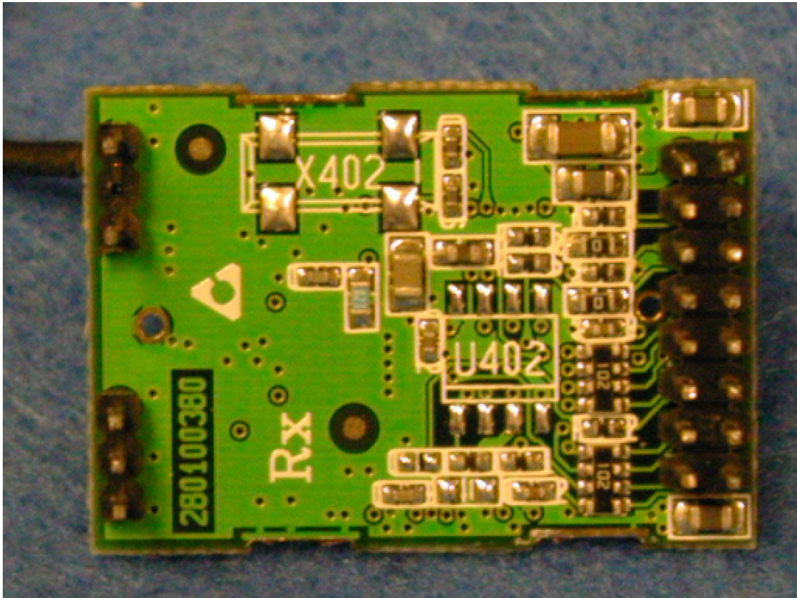
RF Shielding Removed
