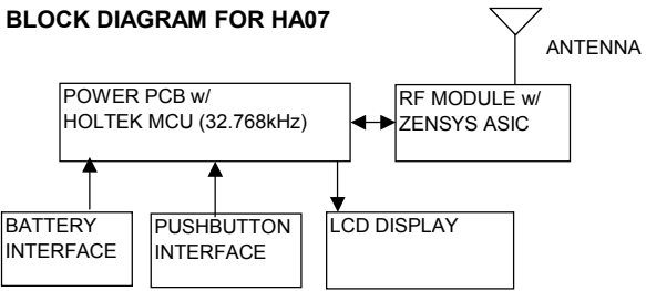
BLOCK DIAGRAM FOR HA07
