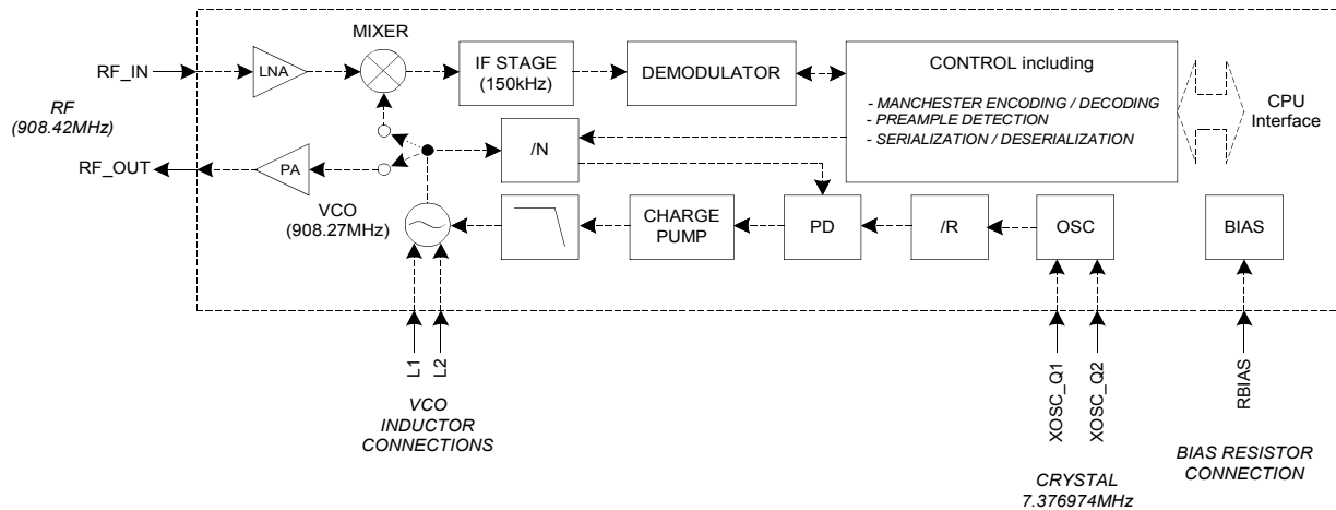
RF Transceiver Block Diagram
