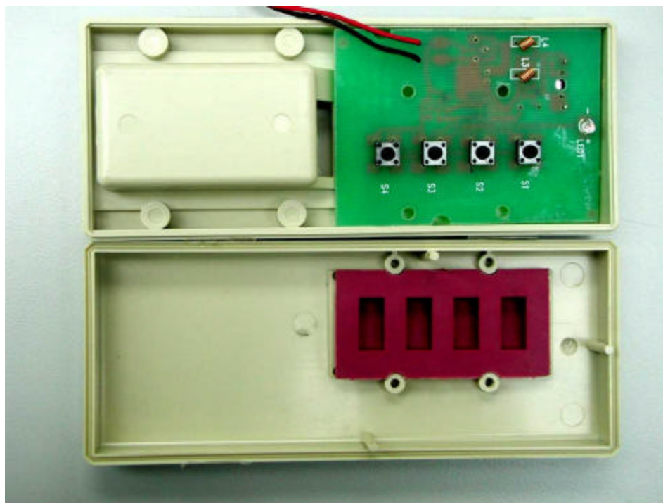
Internal Photo – 3
