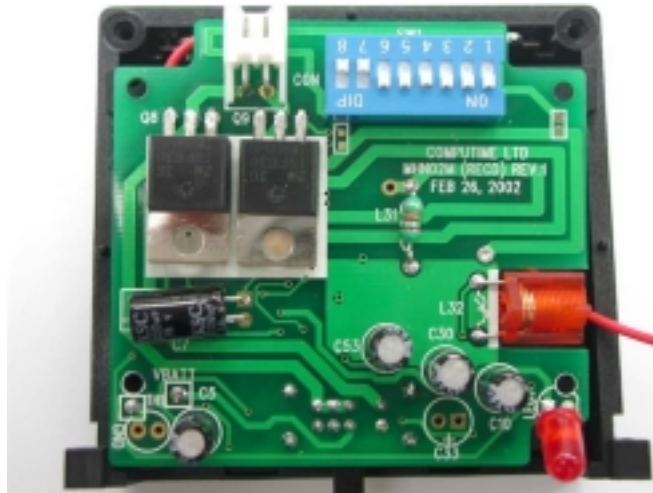
Internal Photo – 3
