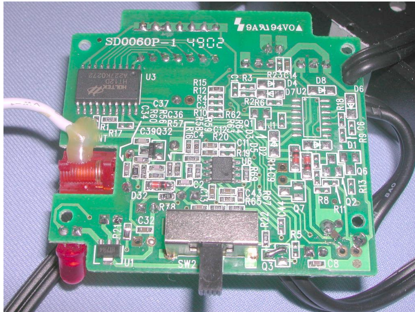
Internal Photo – 4
