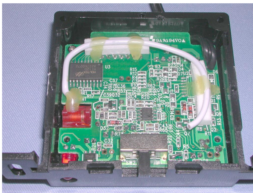
Internal Photo - 2
