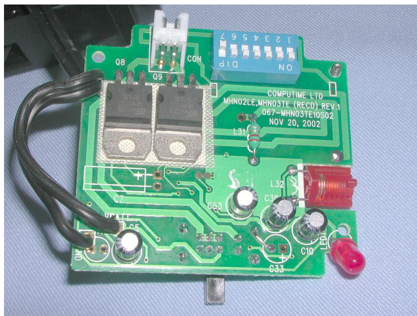
Internal Photo – 5
