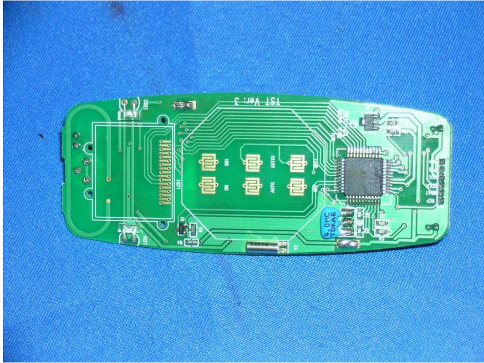
Internal Photo - 6
