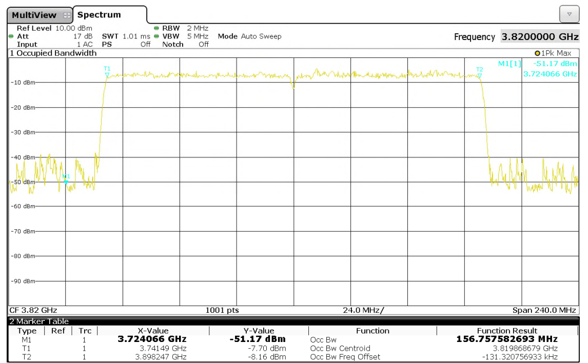
Figure 216: 99% Occupied Bandwidth, 2cc-3a (OBW=80MHz+80MHz), 256QAM_TM3.1a, High Channel, TX Port 17
