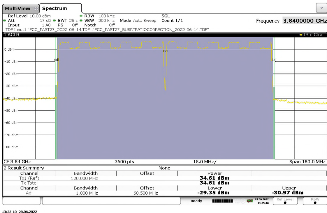
Figure 237: Out-of-Band Emission, 2cc-2b (OBW=60MHz+60MHz), High Channel, 16QAM_TM3.2, TX Port 24
