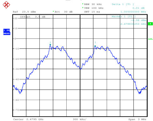
DH1_High 1.005MHz
