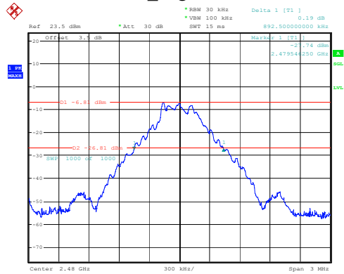
DH1_High 0.893MHz
