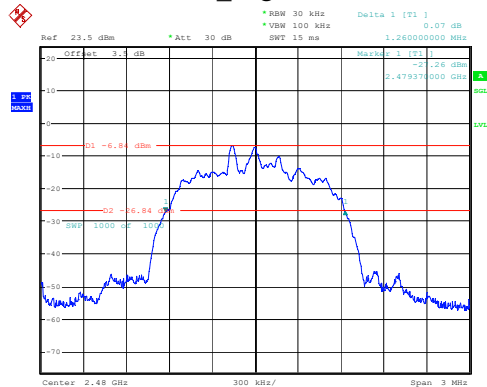
3DH1_High 1.260MHz
