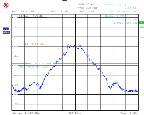
DH1_Low 0.893MHz
