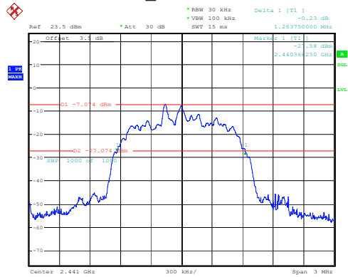
2DH1_Middle 1.264MHz
