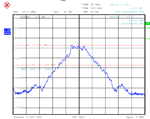
DH1_Middle 0.893MHz
