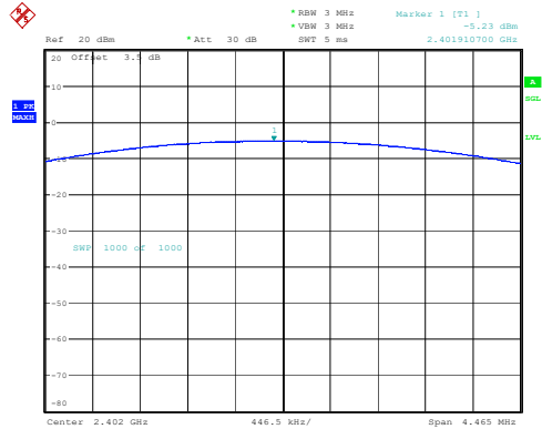
DH1_Low -5.23dBm
