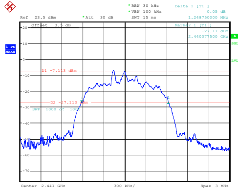
3DH1_Middle 1.249MHz
