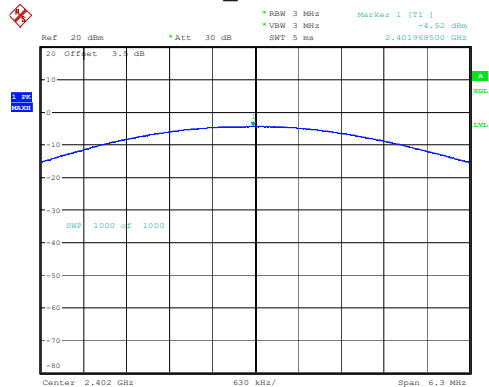
2DH1_Low -4.52dBm
