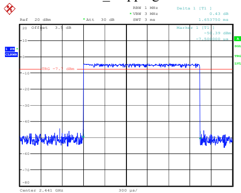
2DH3_Hopping 1.654ms
