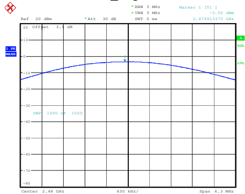
2DH1_High -3.50dBm
