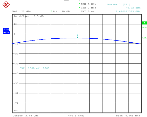
DH1_High -4.22dBm
