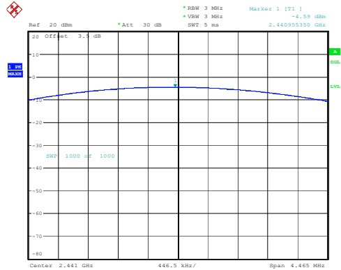
DH1_Middle -4.59dBm
