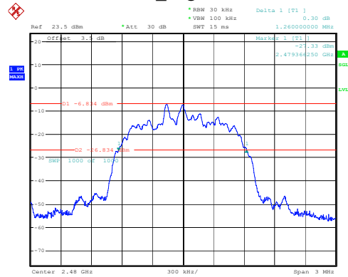
2DH1_High 1.260MHz
