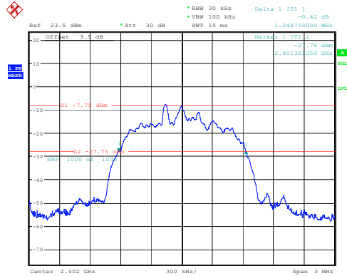
3DH1_Low 1.249MHz
