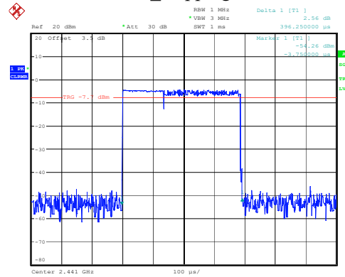
2DH1_Hopping 0.396ms
