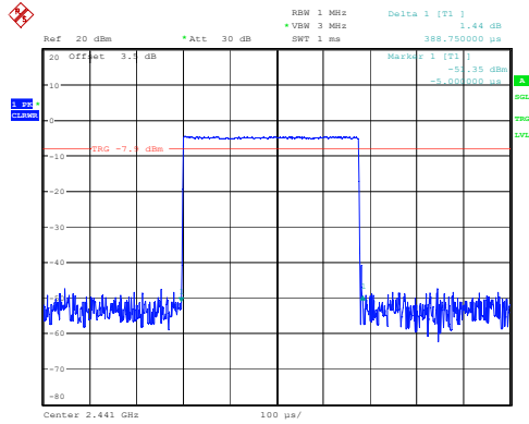
DH1_Hopping 0.389ms
