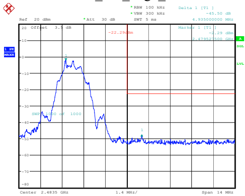
BLE_2M_High_Channel
