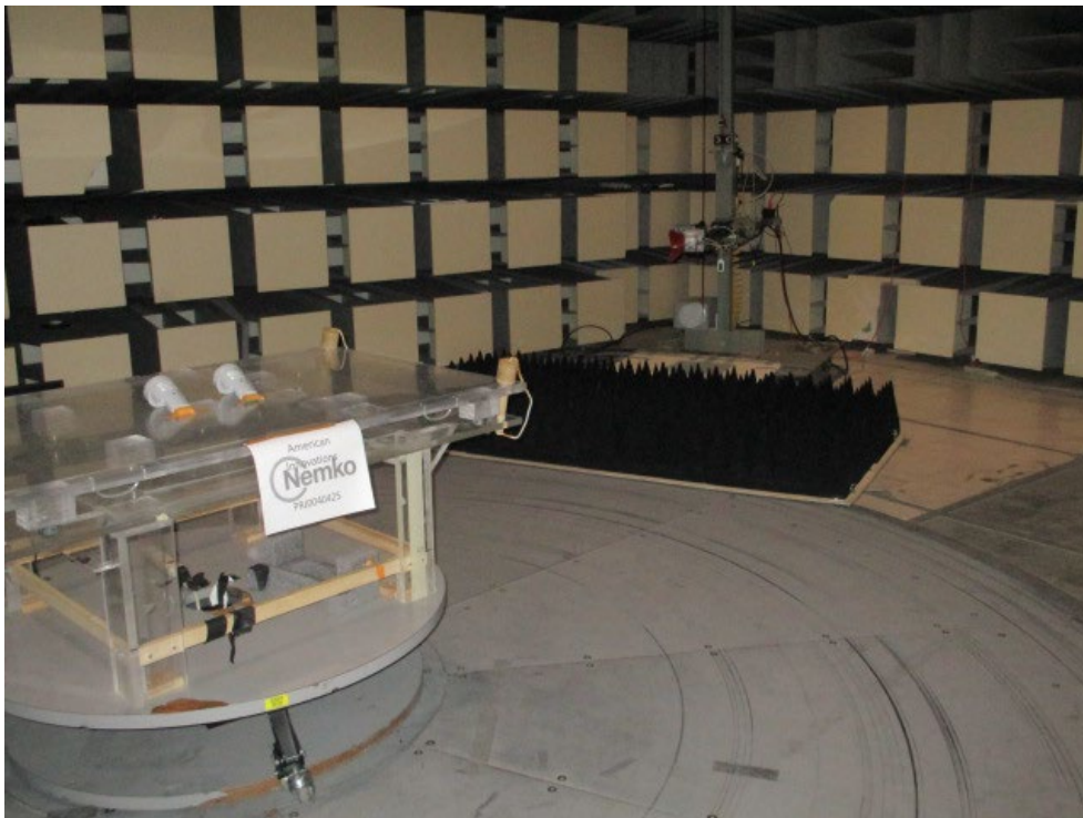
Radiated Emissions, 1 MHz to 18 GHz
