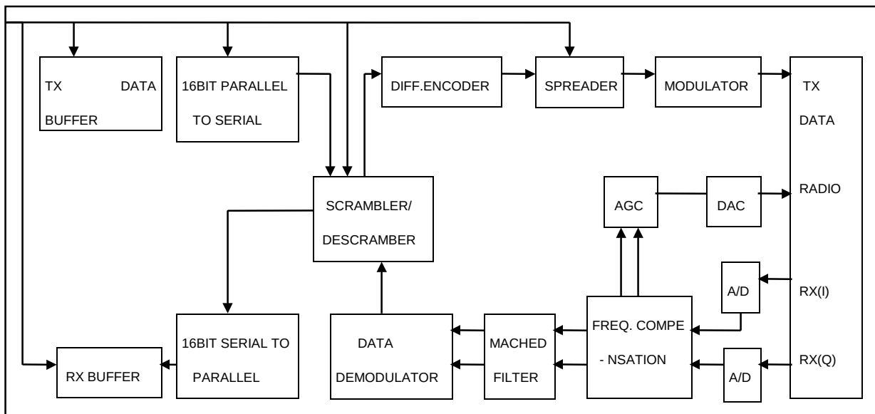
DCT Spread Spectrum Engine Block Diagram
