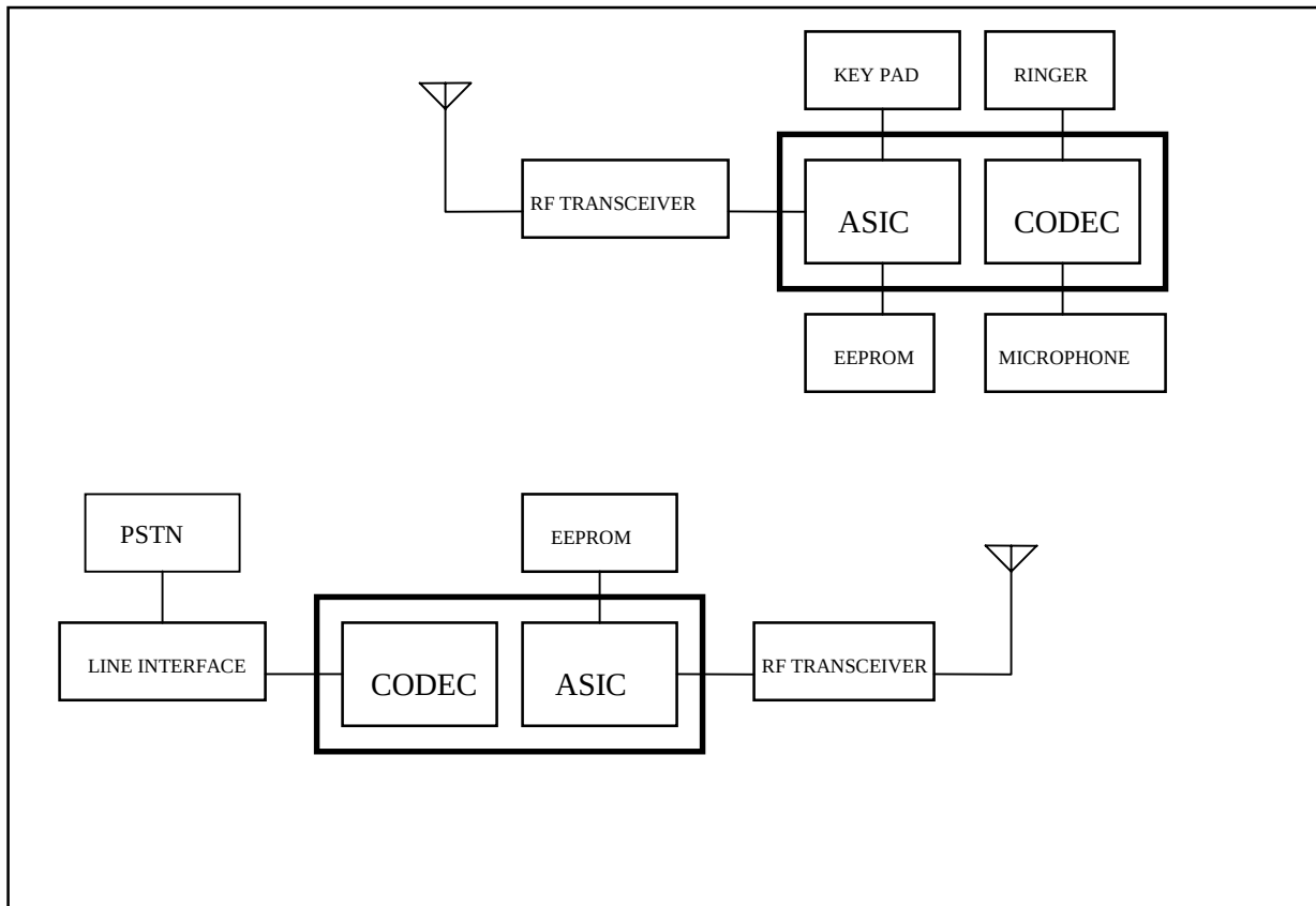
IS - 901 System Architecture
