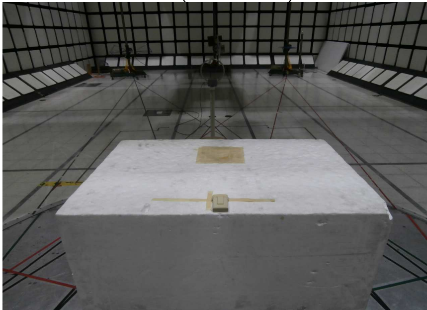
RADIATED REAR PHOTO (BELOW 30MHz)
