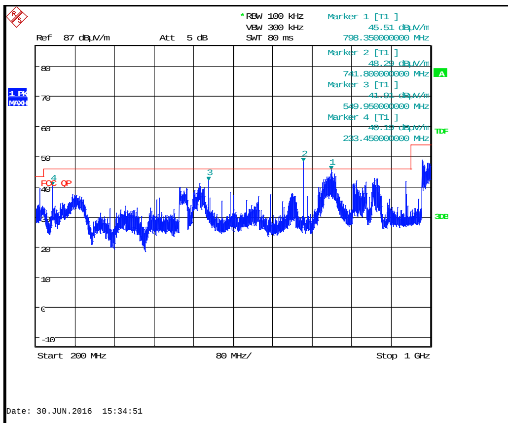
BTLE Tx 2442 MHz : 200 MHz to 1000 MHz
