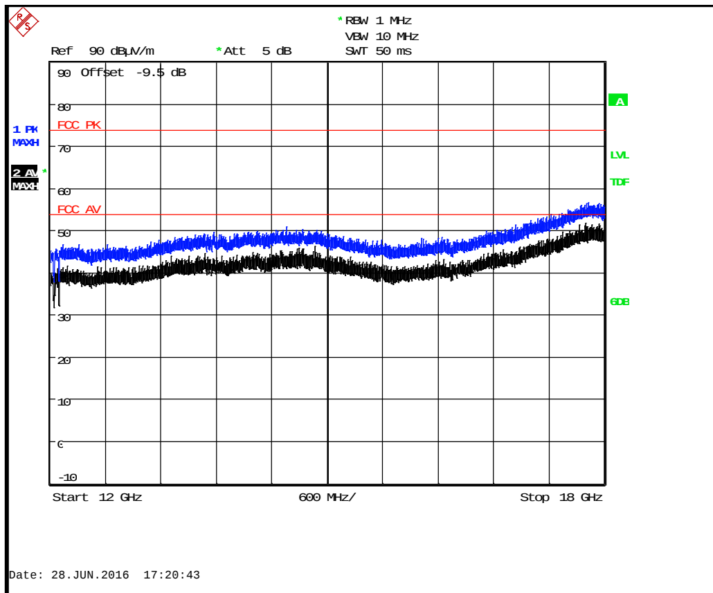
BTLE Tx 2442 MHz : 12 GHz to 18 GHz
