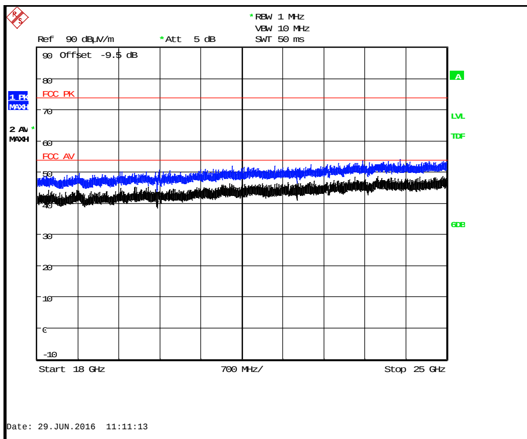
BTLE Tx 2402 MHz: 18 GHz to 25 GHz
