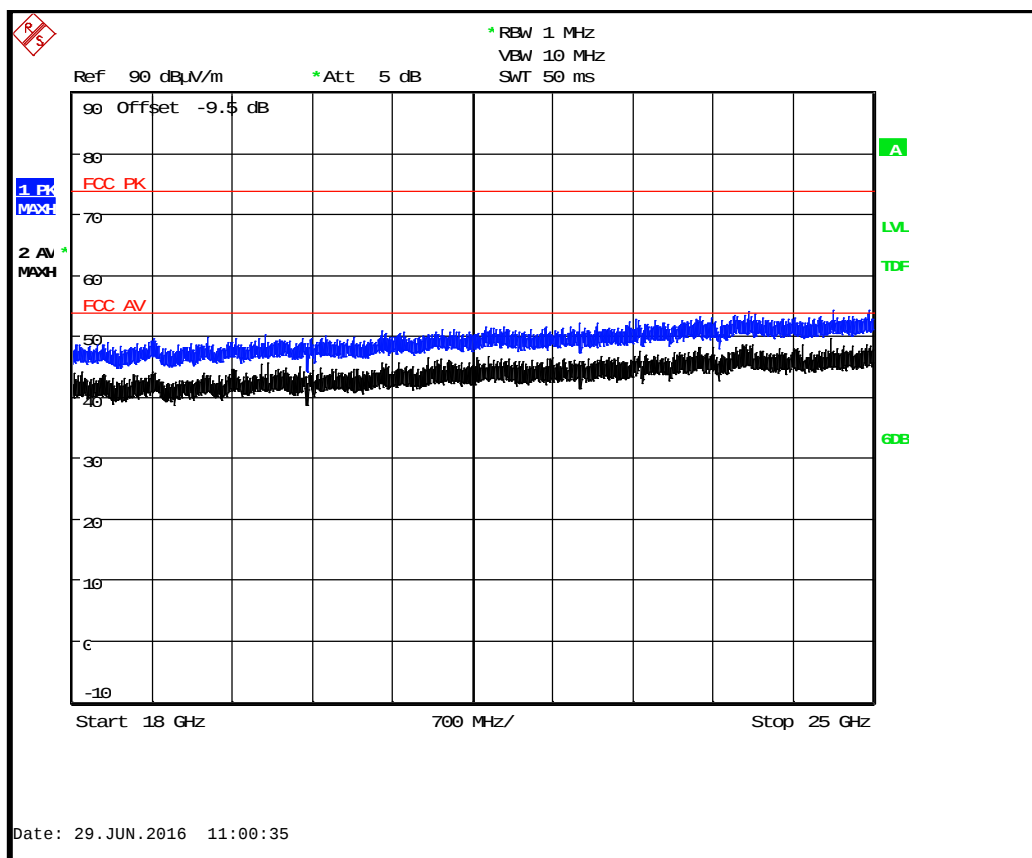
BTLE Tx 2480 MHz: 18 GHz to 25 GHz
