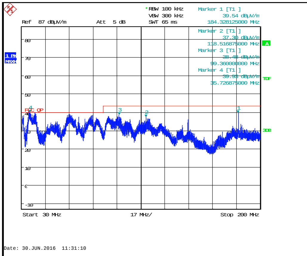
BTLE Tx 2402 MHz : 30 MHz to 200 MHz
