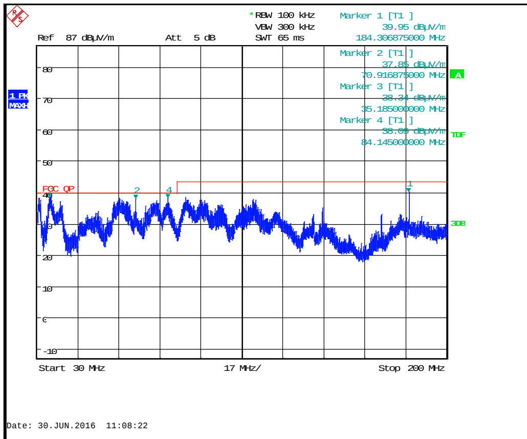
BTLE Tx 2480 MHz : 30 MHz to 200 MHz
