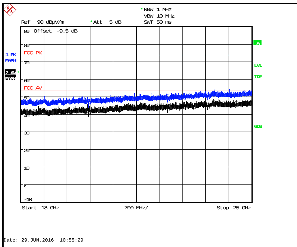
BTLE Tx 2442 MHz: 18 GHz to 25 GHz
