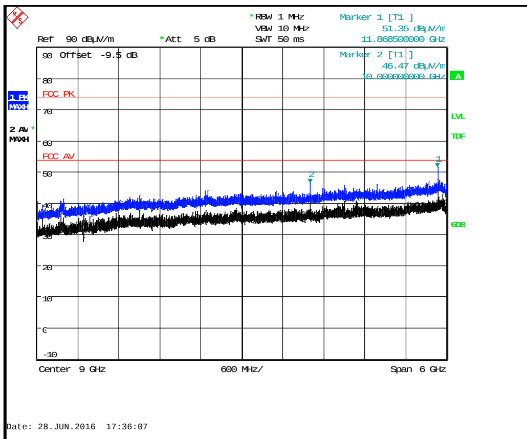
BTLE Tx 2402 MHz : 6 GHz to 12 GHz
