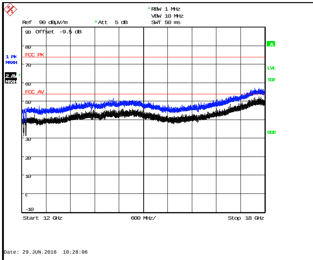
BTLE Tx 2480 MHz : 12 GHz to 18 GHz
