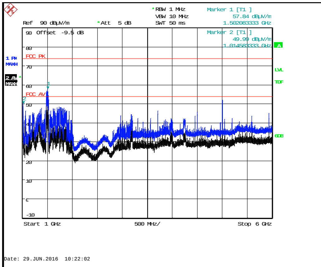
BTLE Tx 2480 MHz : 1 GHz to 6 GHz
