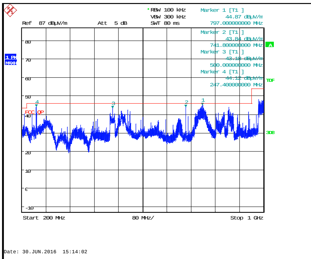
BTLE Tx 2402 MHz : 200 MHz to 1000 MHz
