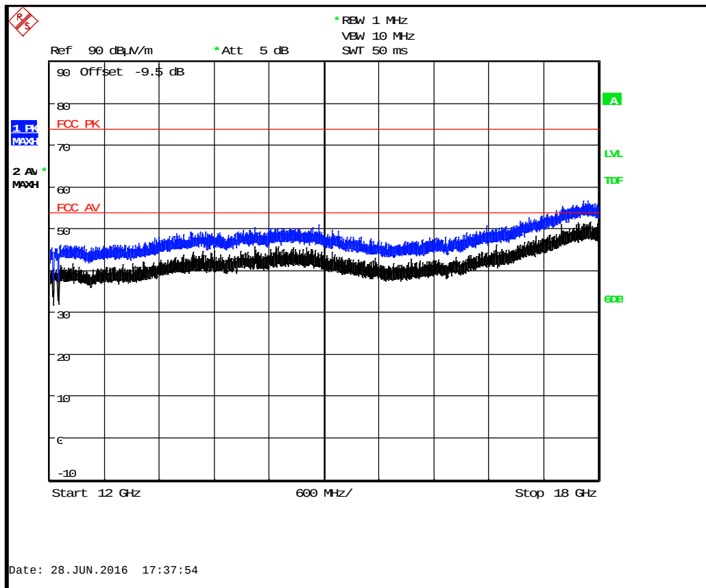
BTLE Tx 2402 MHz : 12 GHz to 18 GHz
