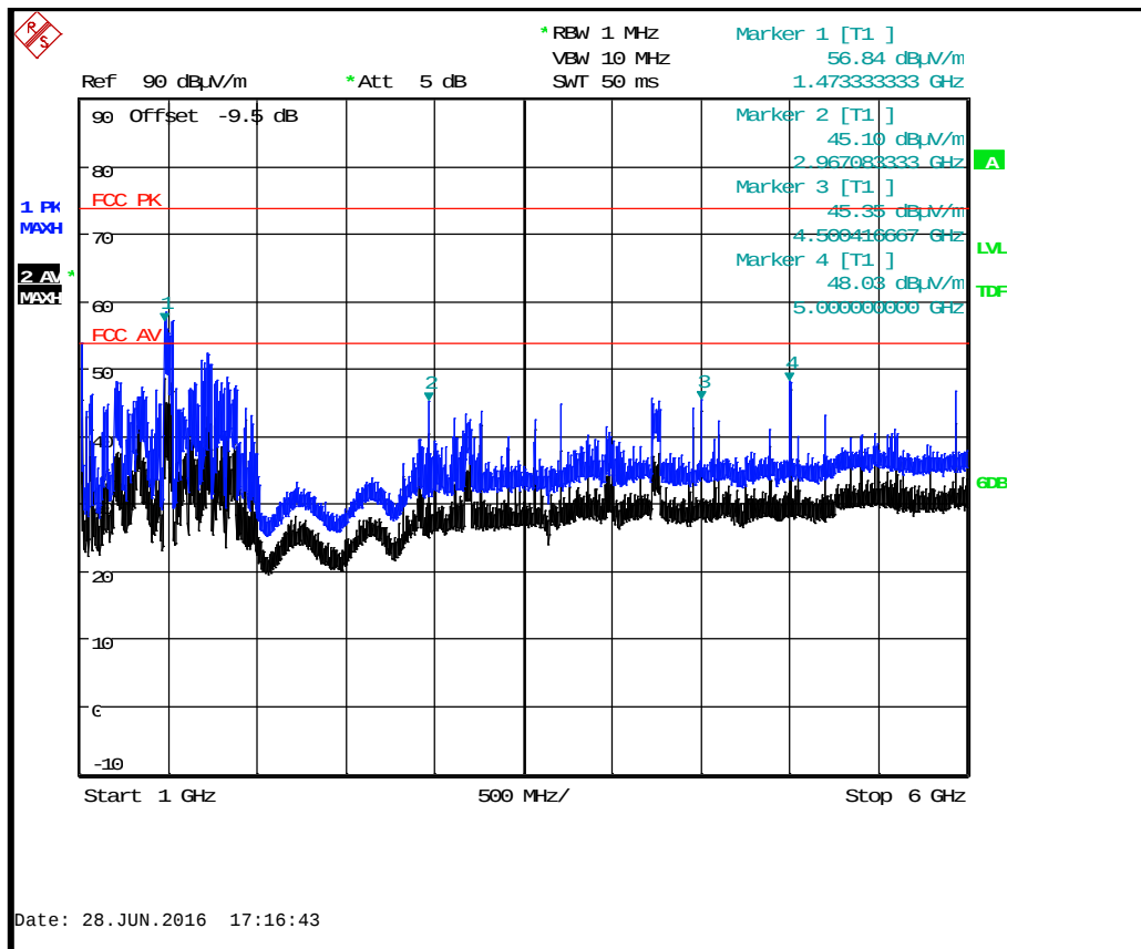
BTLE Tx 2442 MHz : 1 GHz to 6 GHz
