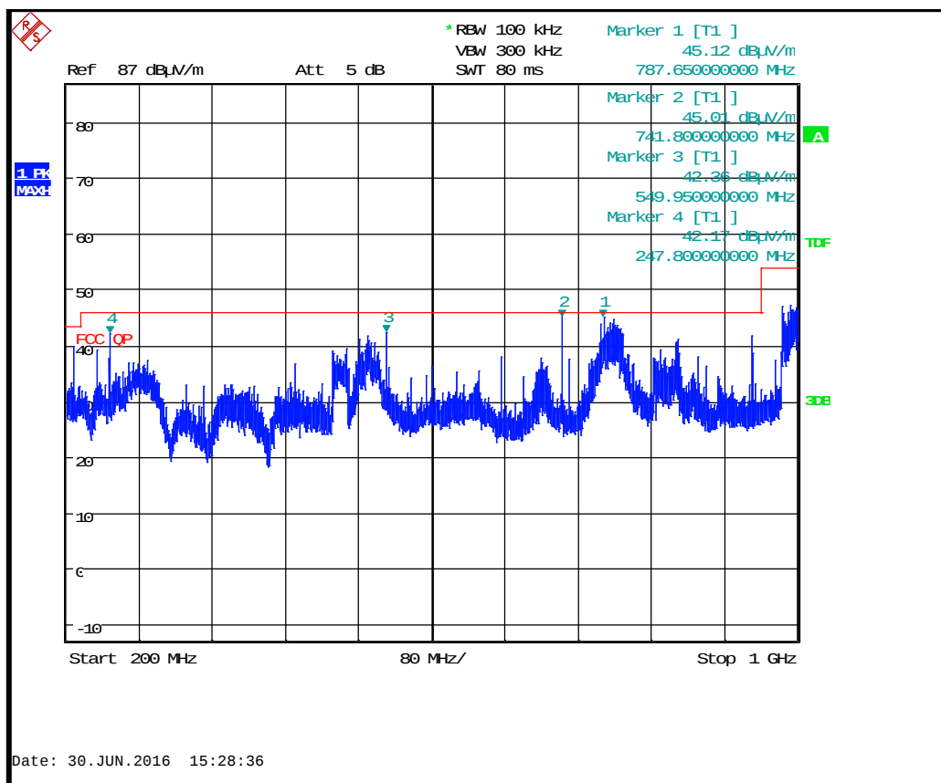
BTLE Tx 2480 MHz : 200 MHz to 1000 MHz
