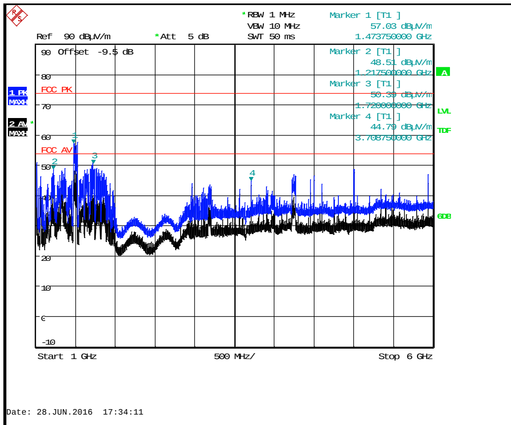
BTLE Tx 2402 MHz : 1 GHz to 6 GHz
