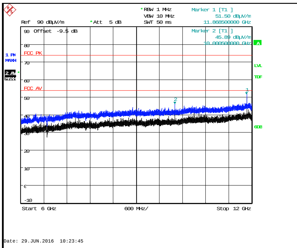
BTLE Tx 2480 MHz : 6 GHz to 12 GHz
