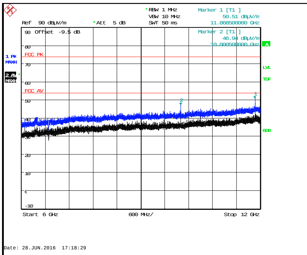
BTLE Tx 2442 MHz : 6 GHz to 12 GHz
