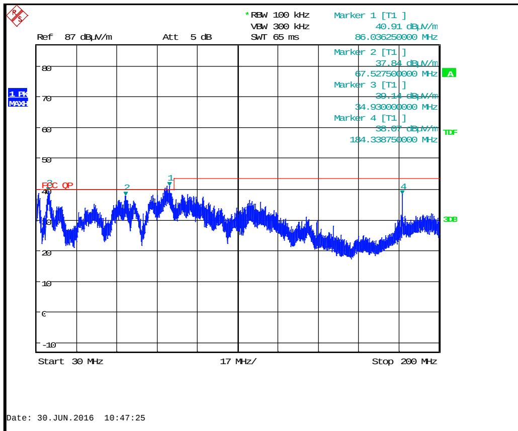
BTLE Tx 2442 MHz : 30 MHz to 200 MHz
