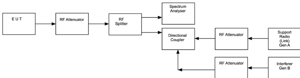
Figure i Test Setup
