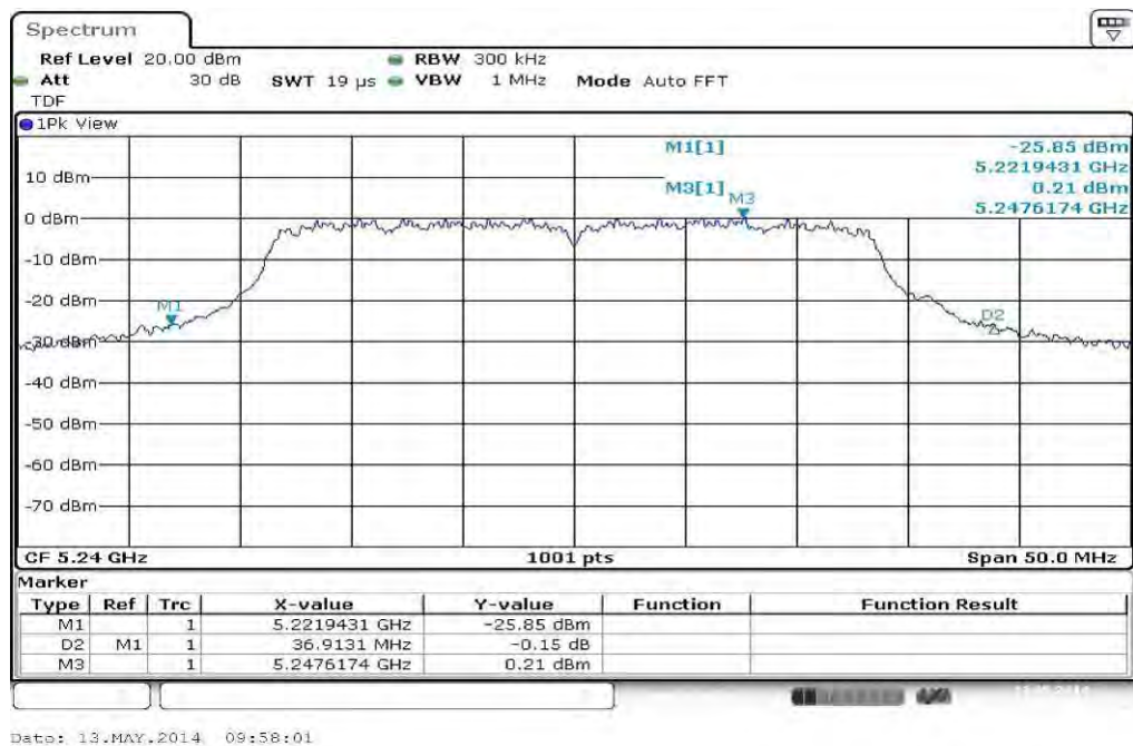
Plot 2: 5240 MHz
