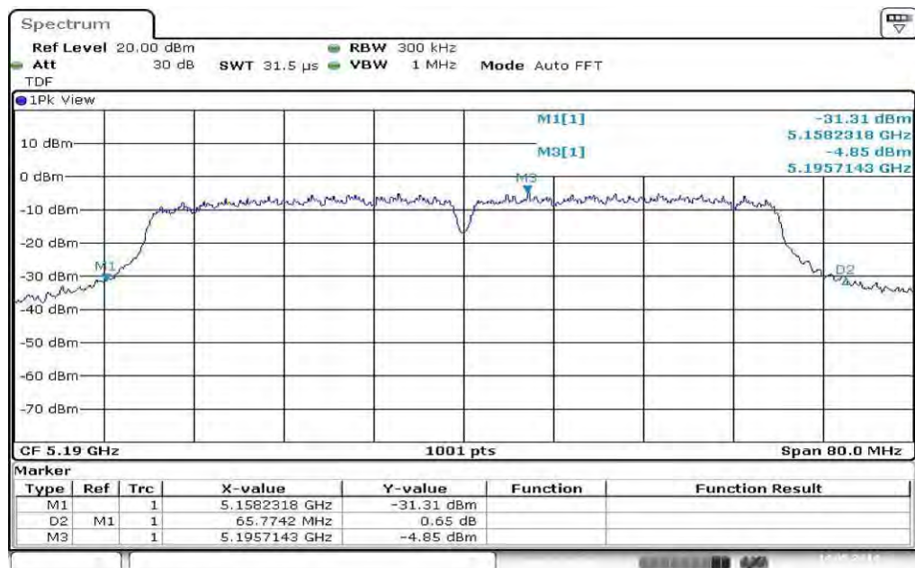
Plot 1: 5190 MHz
