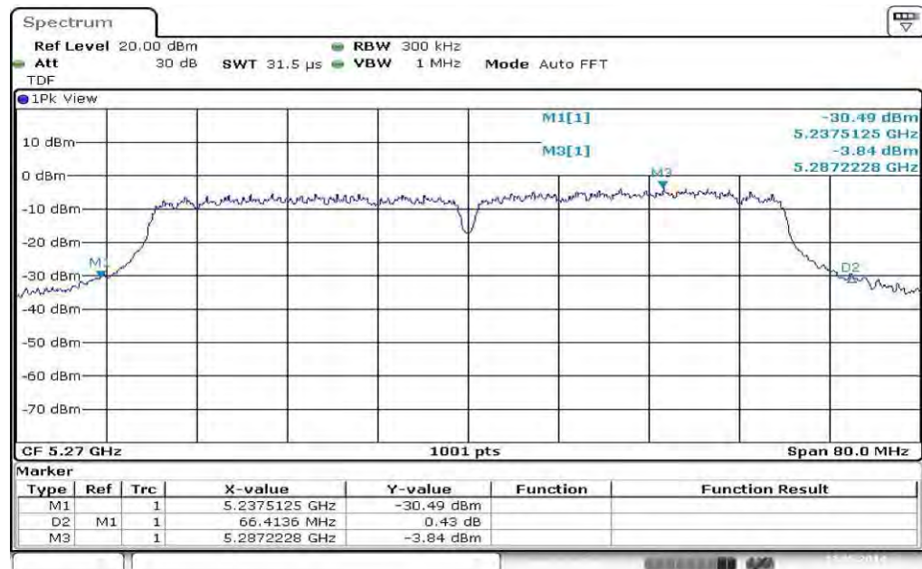
Plot 3: 5270 MHz
