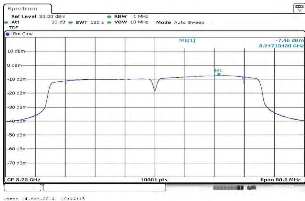
Plot 2: 5230 MHz
