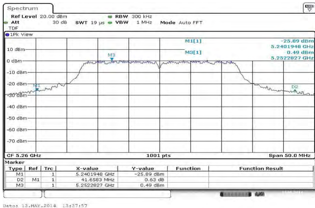
Plot 3: 5260 MHz
