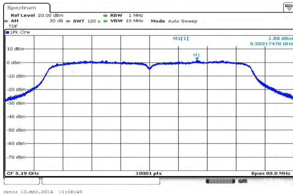
Plot 1: 5190 MHz
