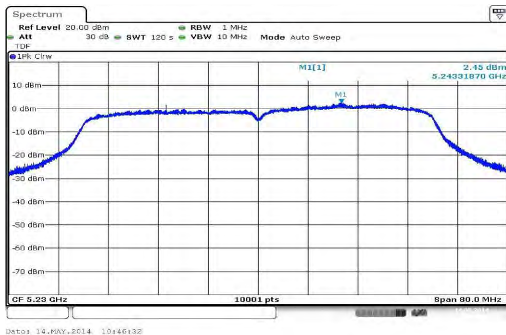
Plot 9: 5230 MHz
