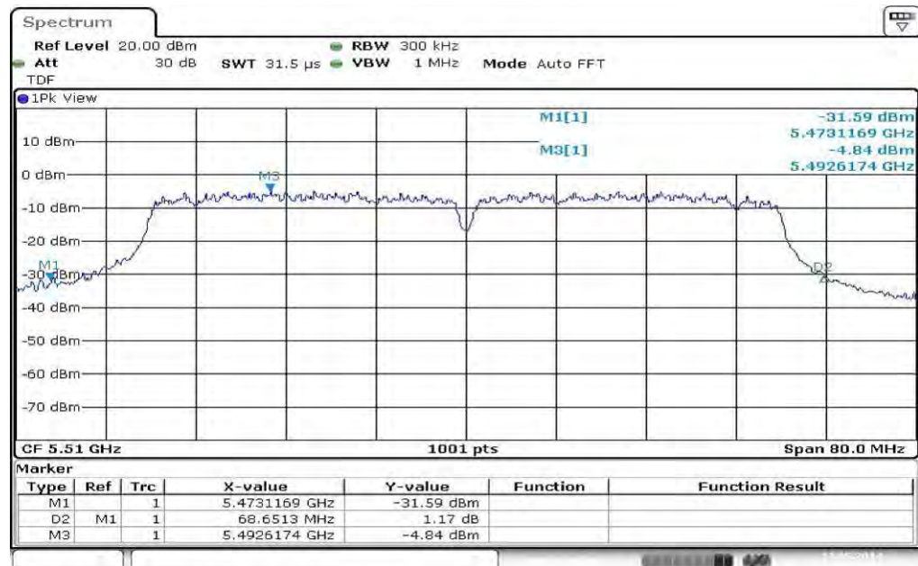
Plot 5: 5510 MHz
