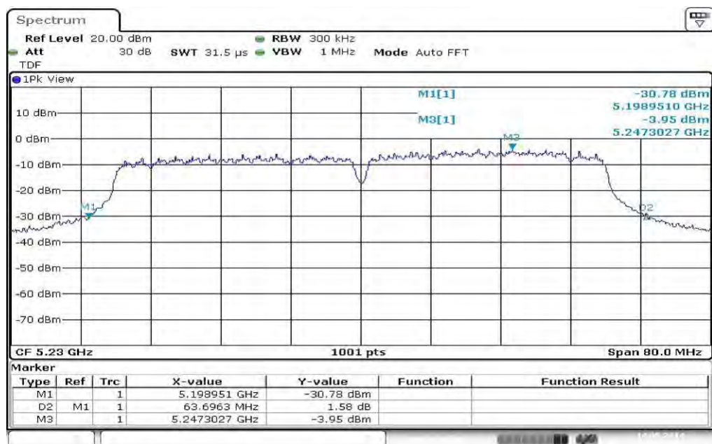
Plot 2: 5230 MHz
