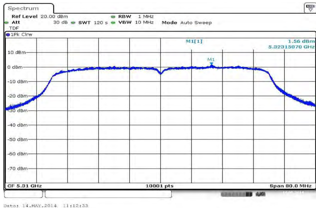
Plot 11: 5310 MHz
