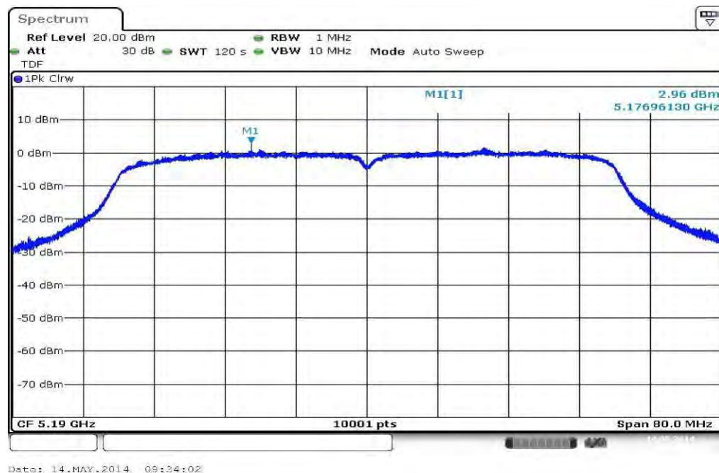
Plot 8: 5190 MHz
