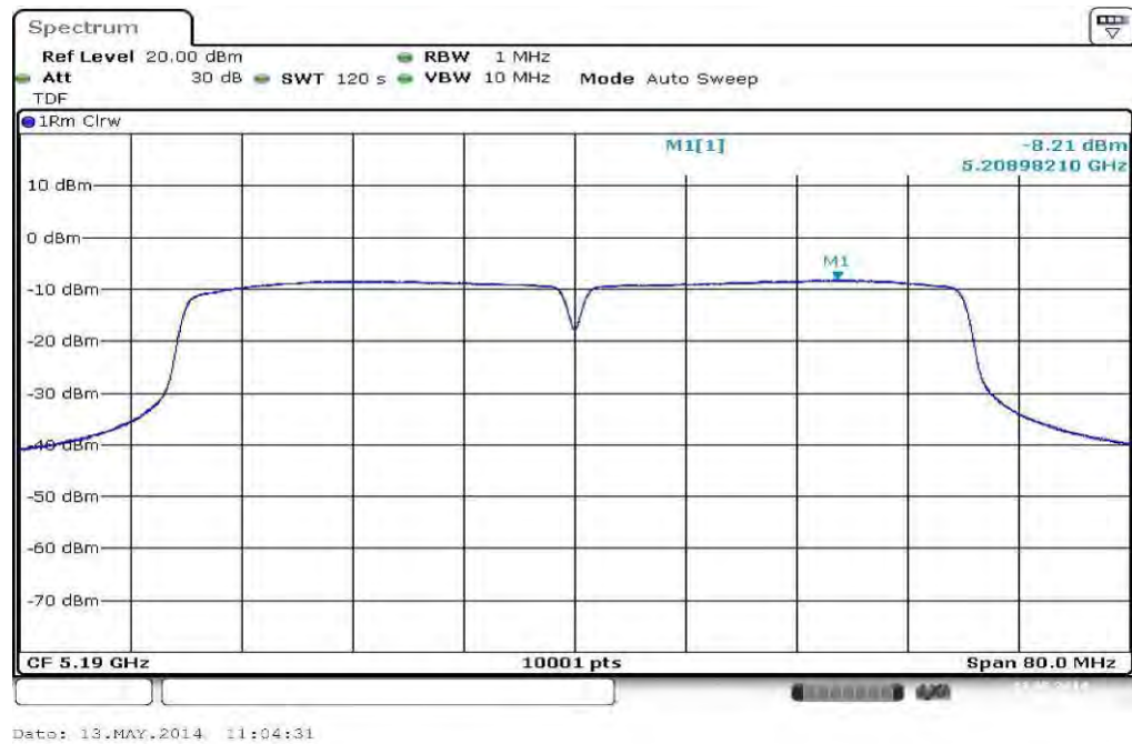
Plot 1: 5190 MHz
