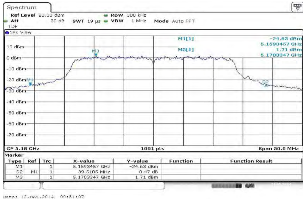
Plot 1: 5180 MHz
