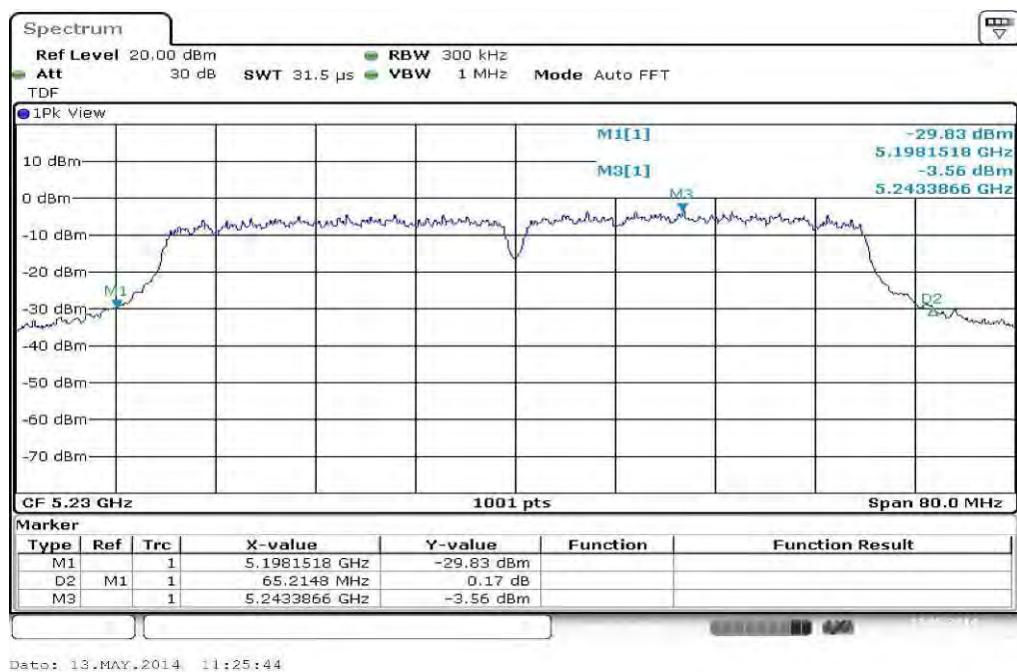
Plot 2: 5230 MHz
