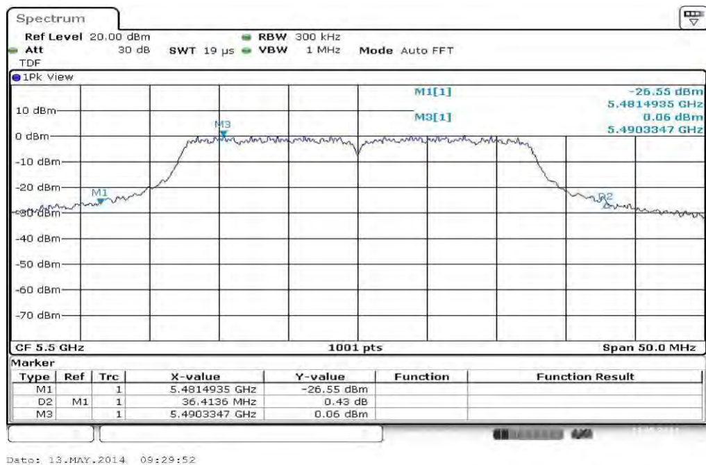
Plot 5: 5500 MHz
