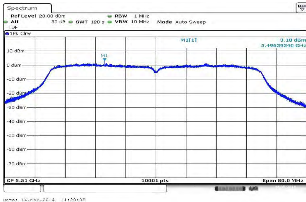
Plot 12: 5510 MHz
