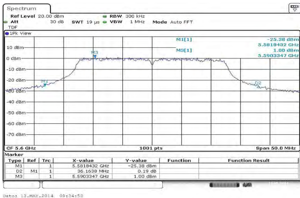
Plot 6: 5600 MHz
