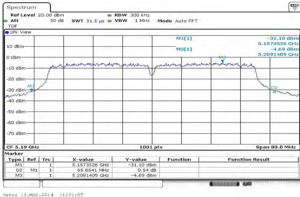
Plot 1: 5190 MHz
