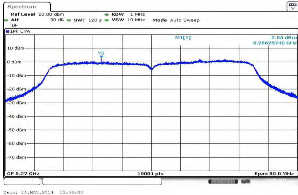
Plot 10: 5270 MHz
