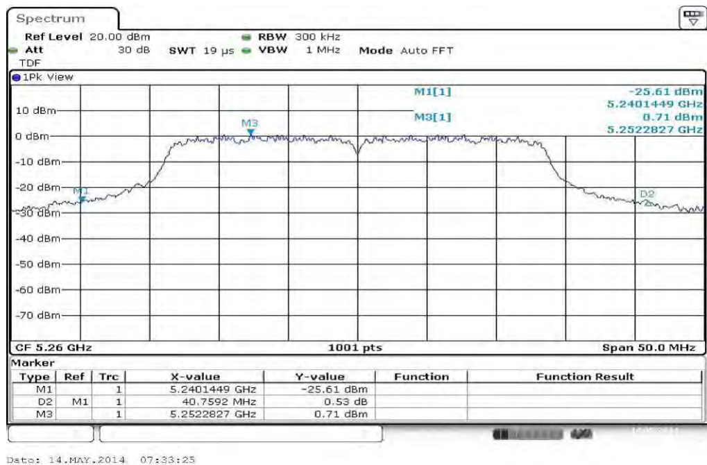
Plot 3: 5260 MHz
