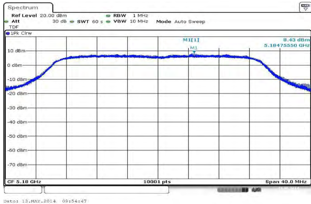
Plot 1: 5180 MHz
