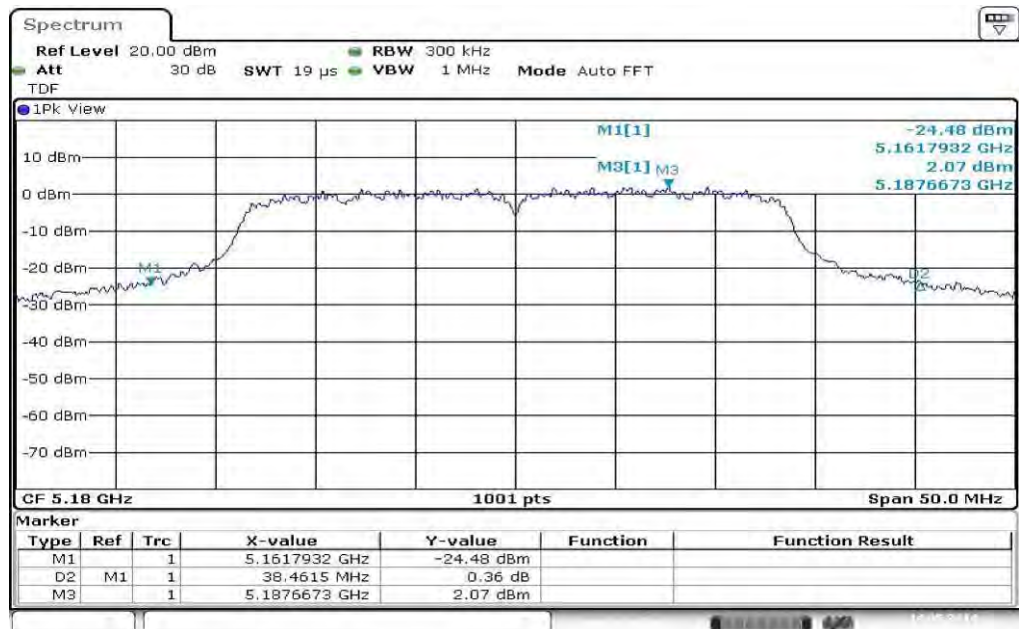
Plot 1: 5180 MHz
