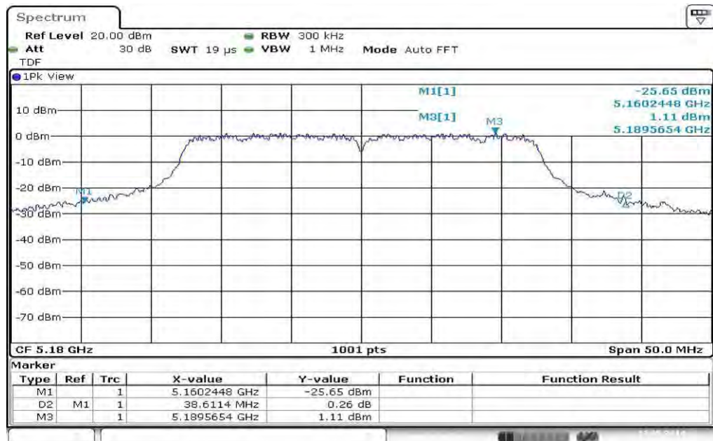
Plot 1: 5180 MHz
