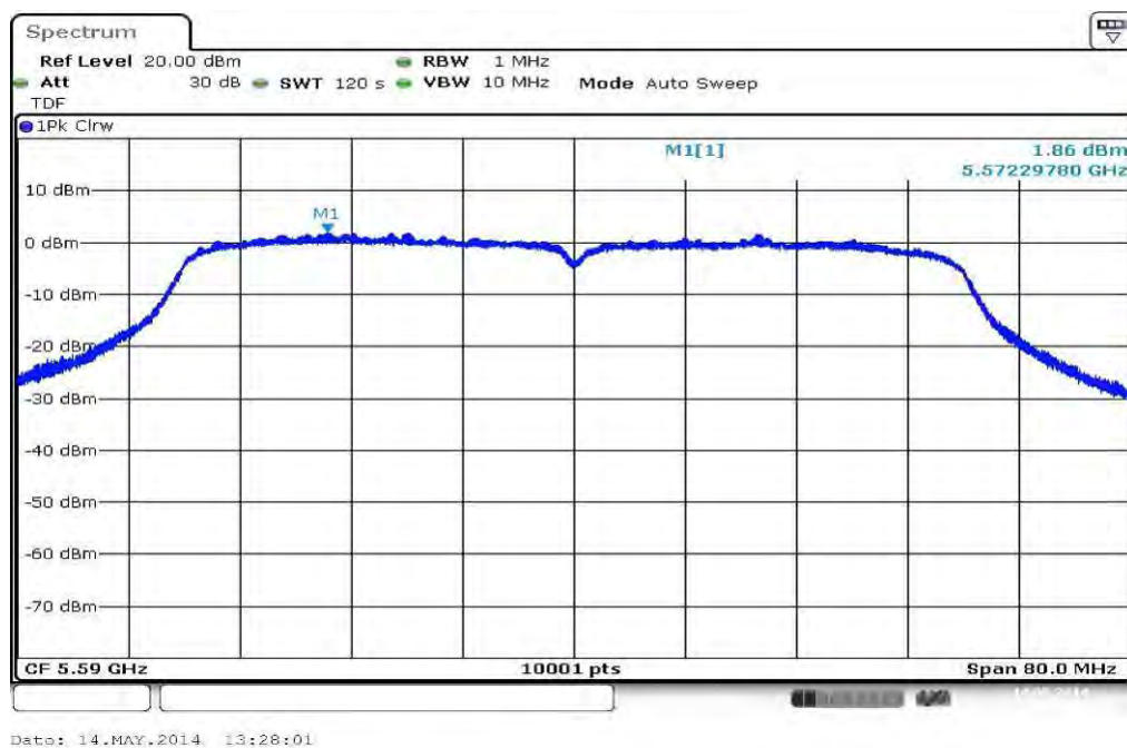
Plot 13: 5590 MHz
