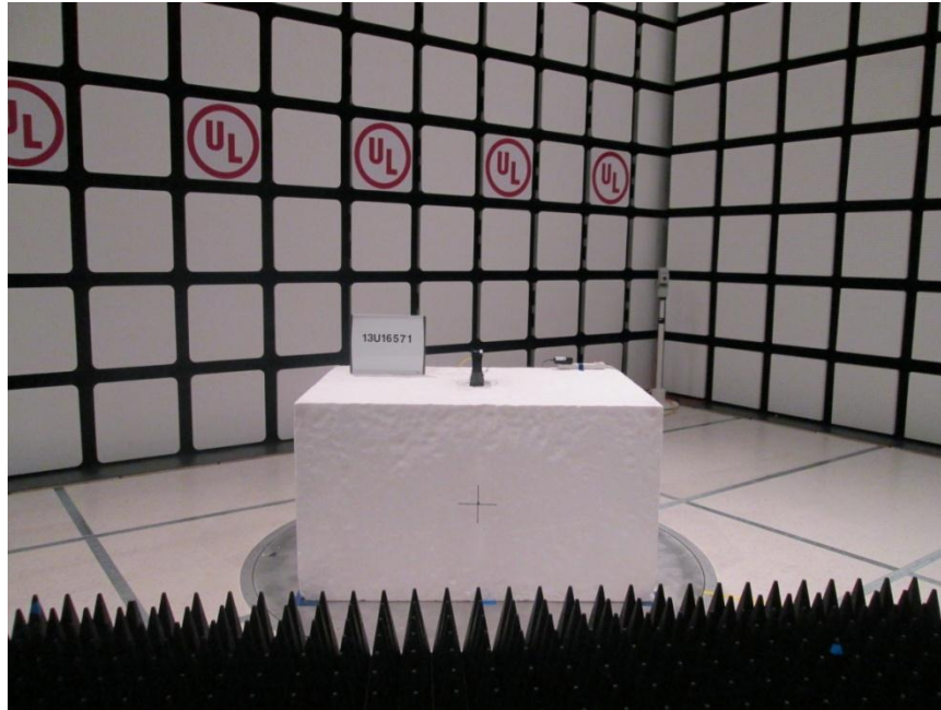
RADIATED FRONT
