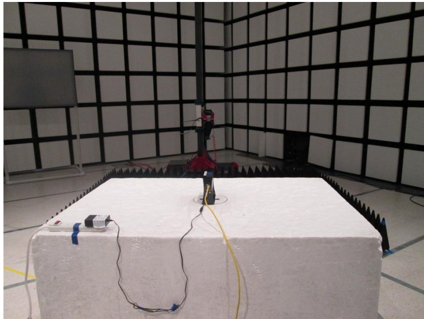
RADIATED BACK
