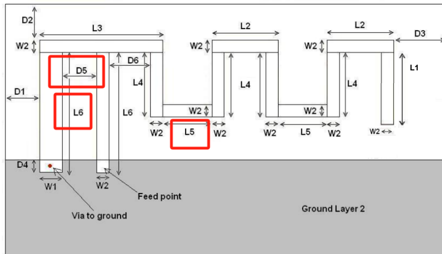
Figure 3: Antenna Dimensions
