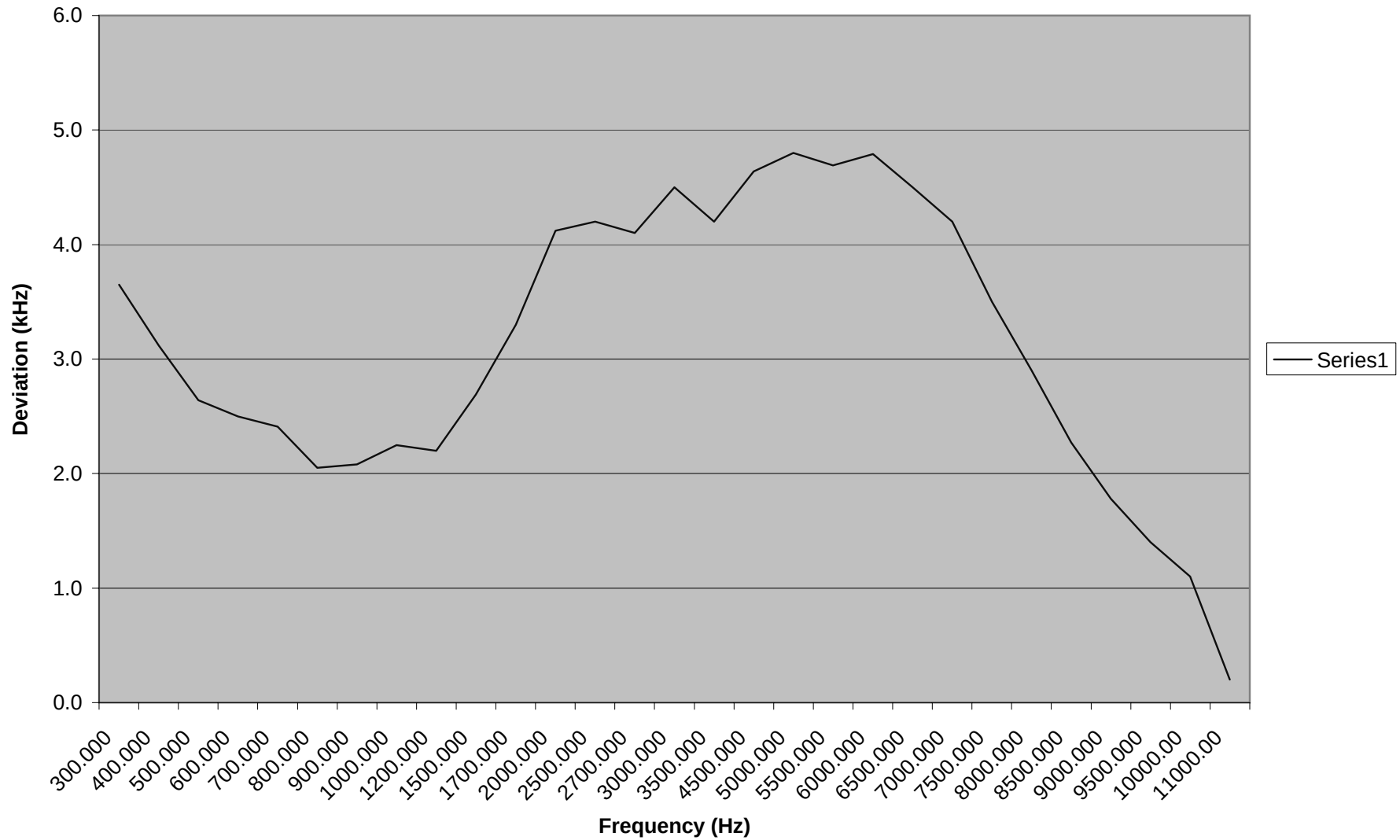
Frequency Response (WM-3210)
