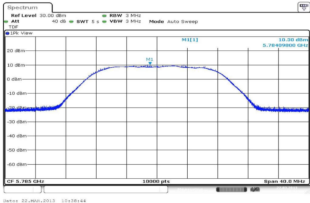
Plot 2: TX mode, 5785 MHz
