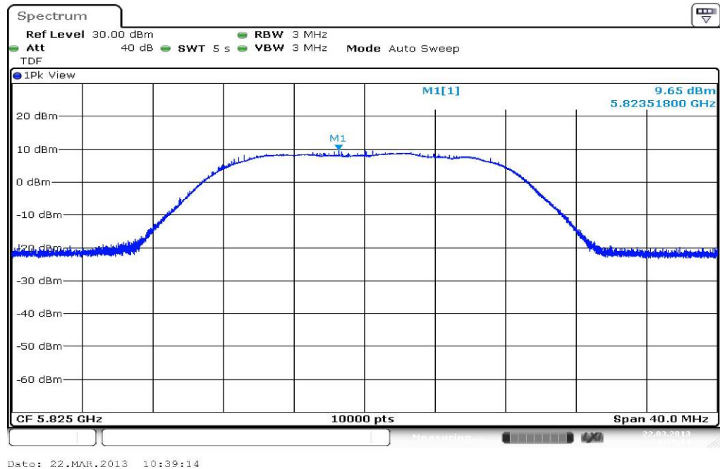
Plot 3: TX mode, 5825 MHz
