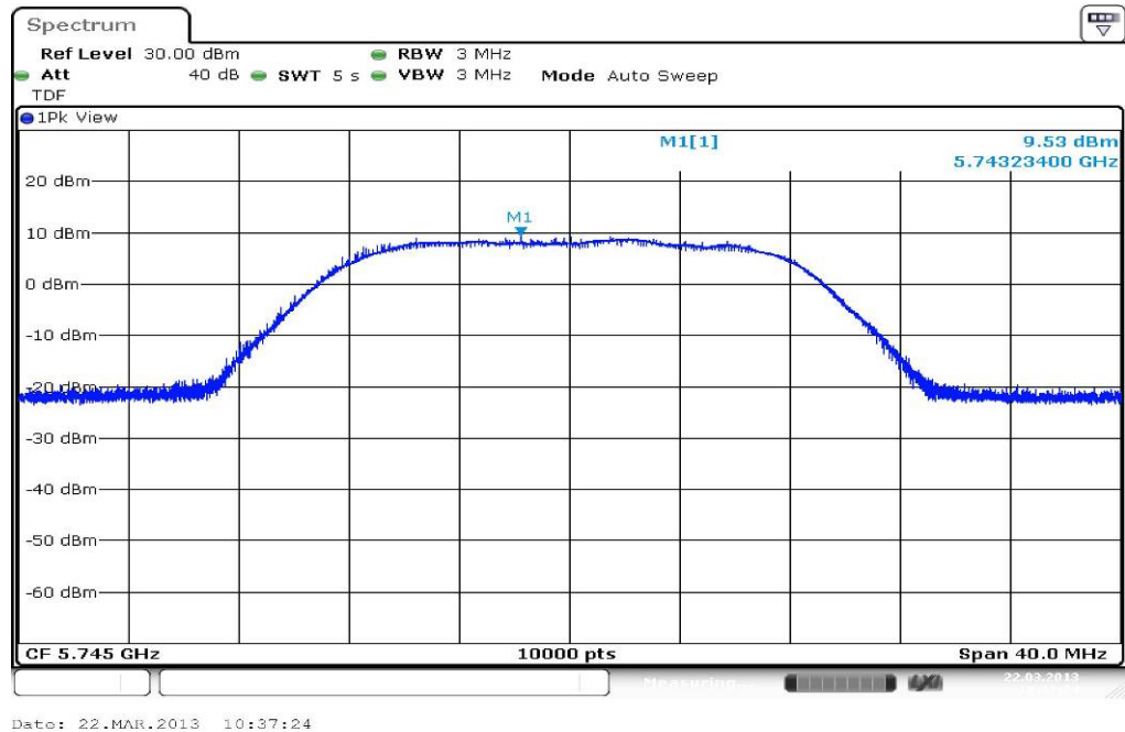
Plot 1: TX mode, 5745 MHz
