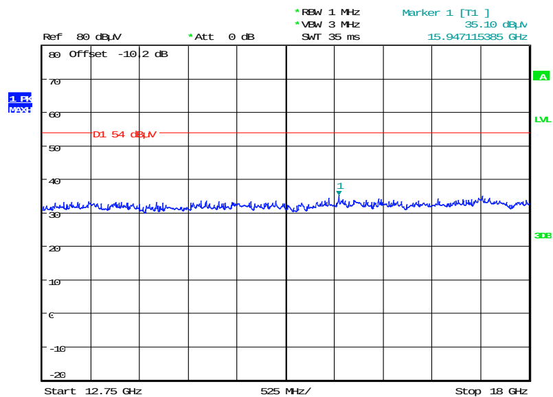
Plot 4: 12.75 GHz to 18 GHz, vertical & horizontal polarization
