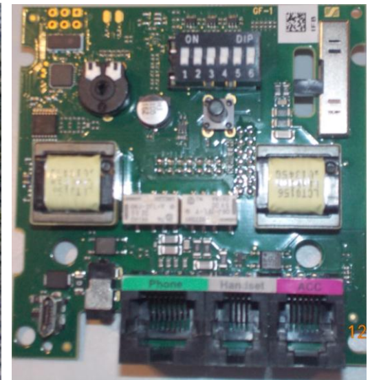
Figure 4.3: New IFB PCB top view in D 10 BS PHONE-US
