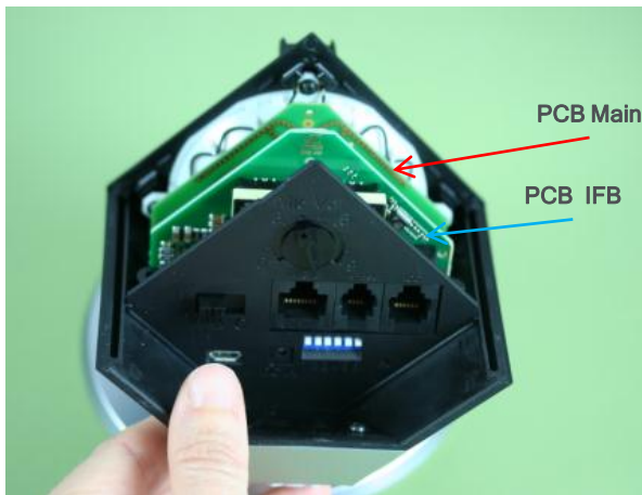
Figure 3.1: Inner side of DW BS-US
