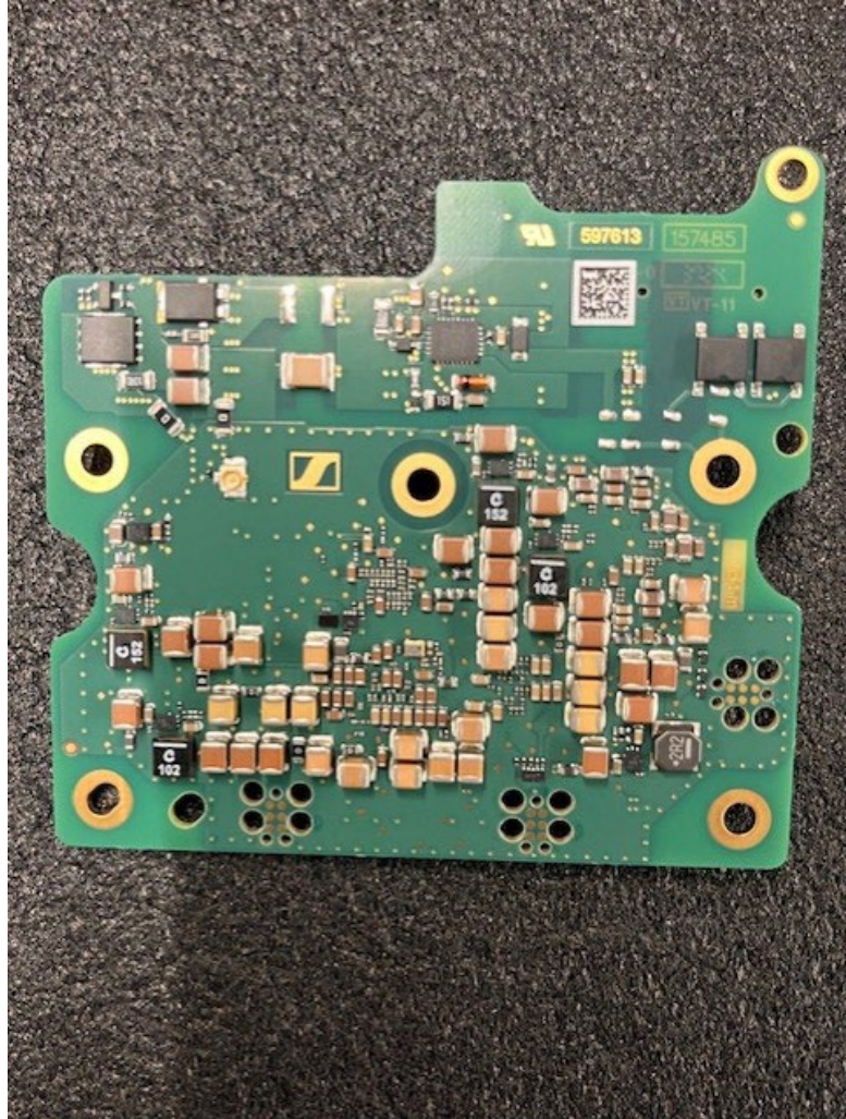
Bottom View (Main PCB)
