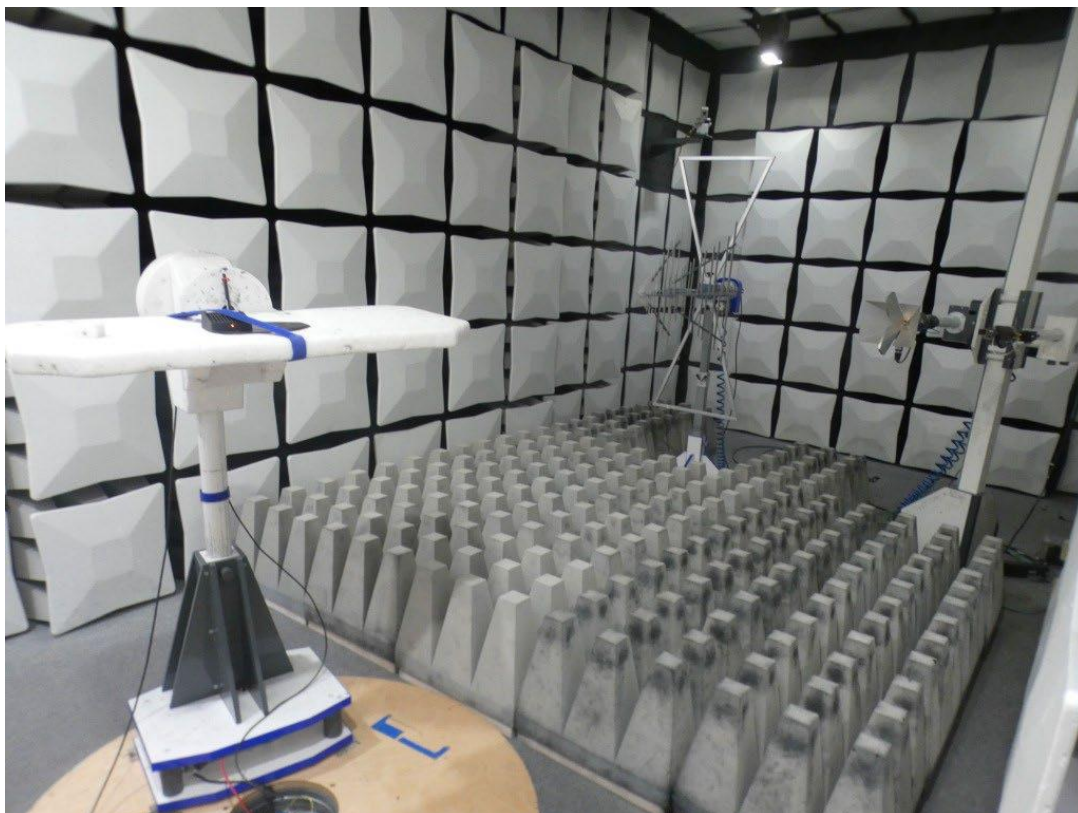
Photo 3: Setup Spurious Emissions Radiated (FAC), > 1\text{GHz}
