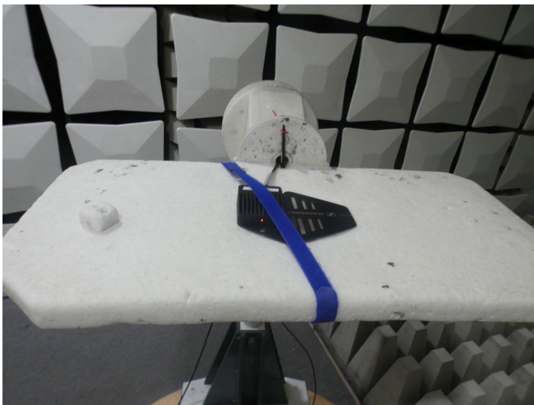
Photo 4: Setup Spurious Emissions Radiated (FAC), > 1\text{GHz} , detail view
