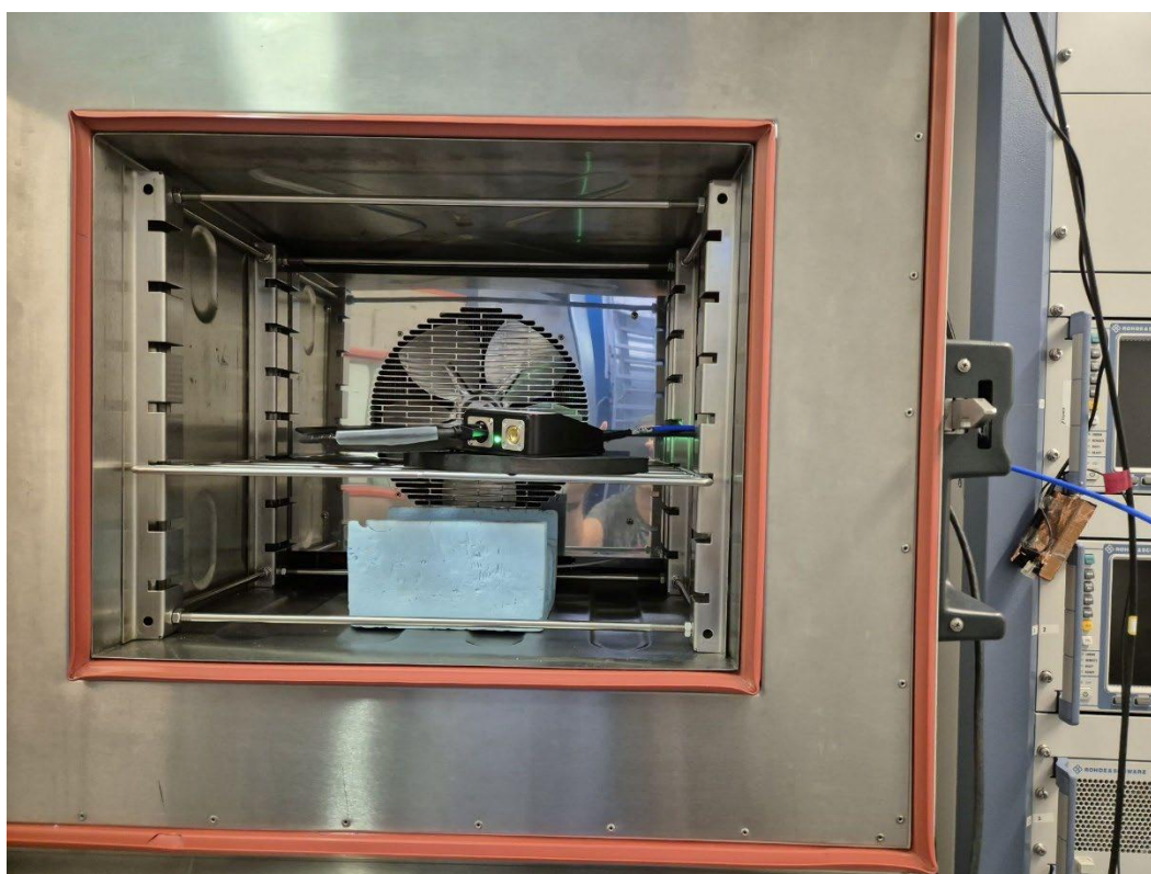
Photo 5: Setup conducted tests, frequency stability in climatic chamber
