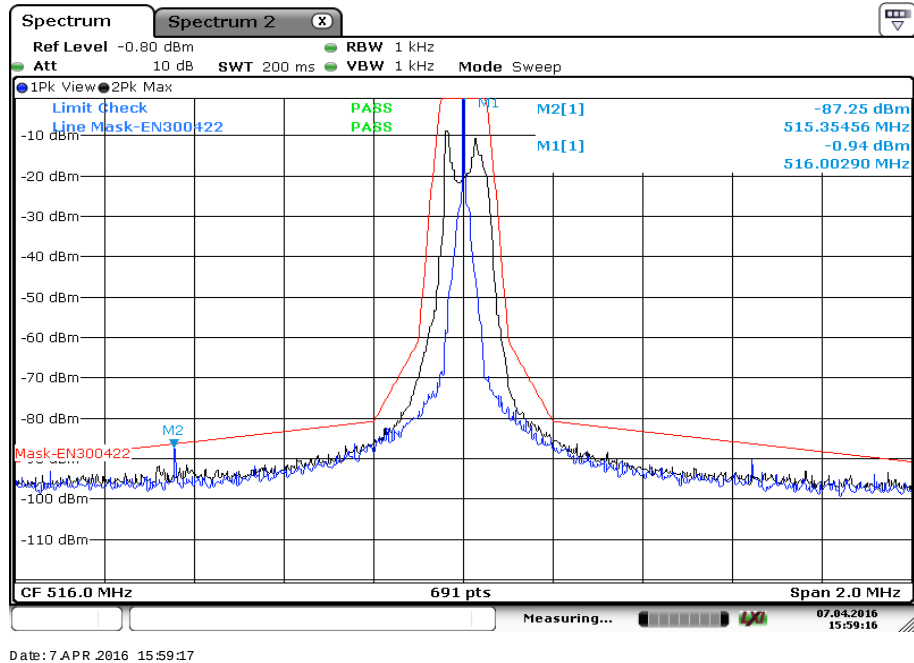
Plot 3: highest channel, unmodulated carrier for reference and modulated carrier
