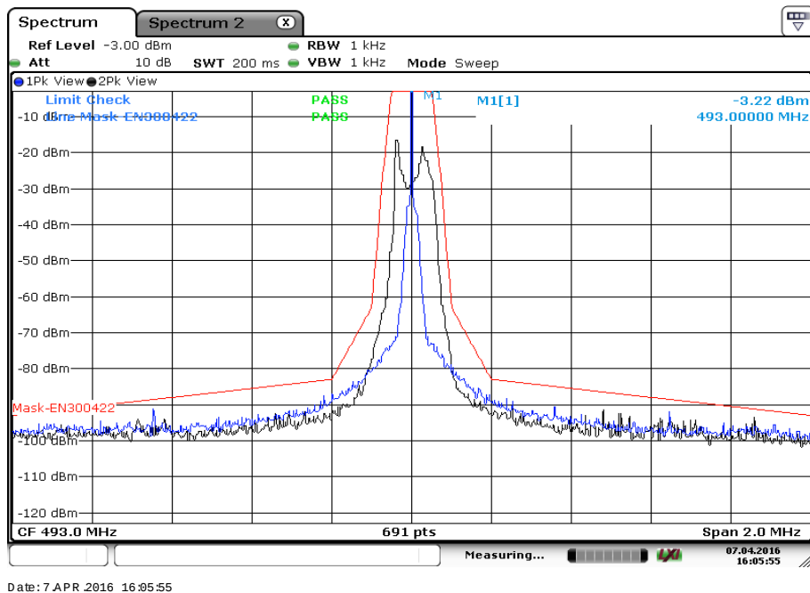
Plot 2: middle channel, unmodulated carrier for reference and modulated carrier
