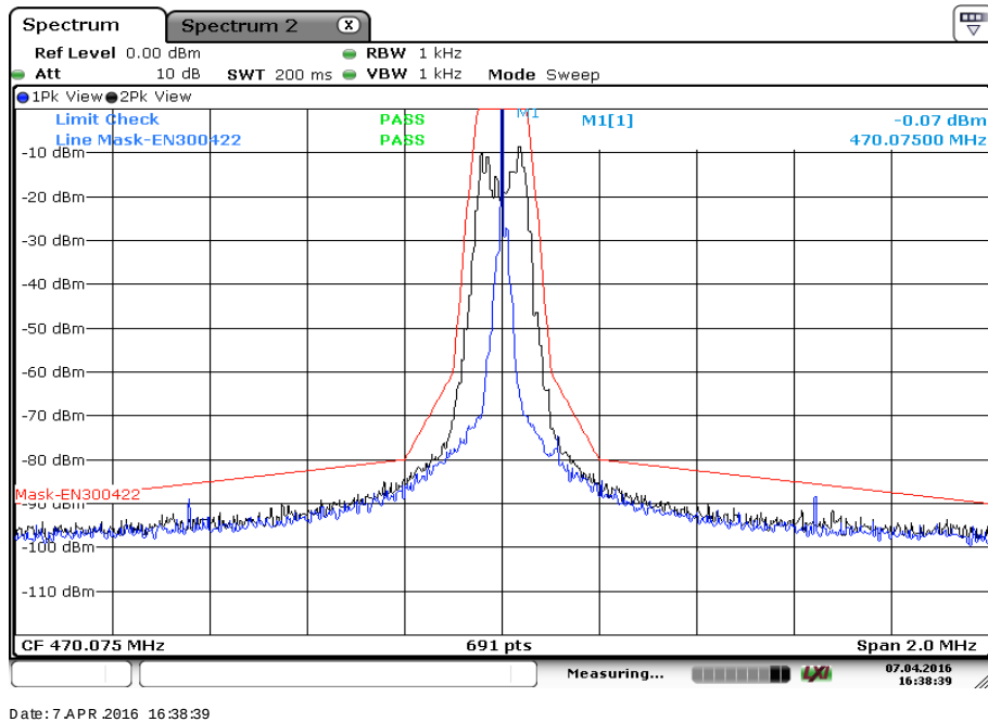
Plot 1: lowest channel, unmodulated carrier for reference and modulated carrier
