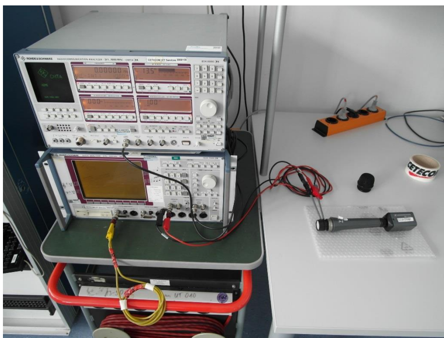
Photo 10: audio analyzer
