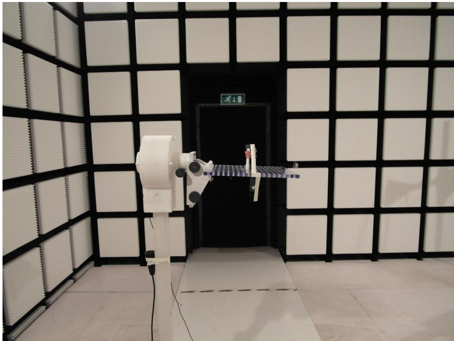
Photo 4: chamber A
