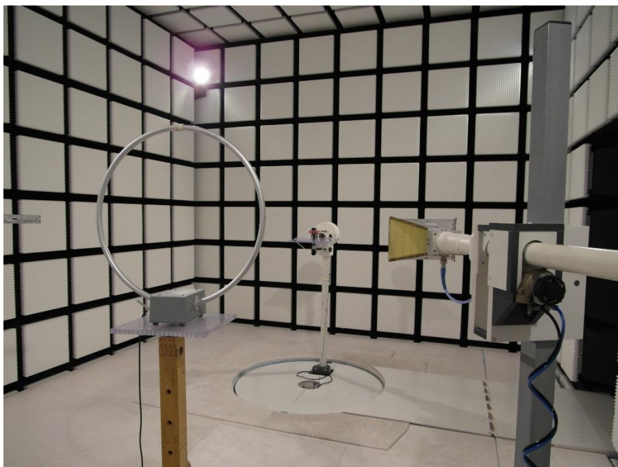
Photo 7: chamber A
