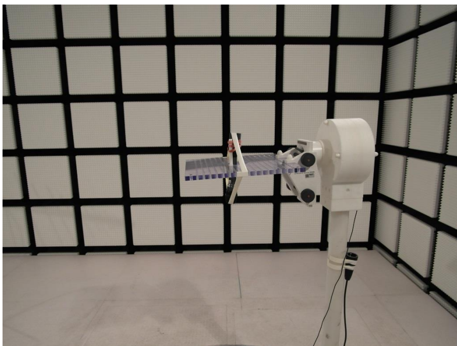
Photo 2: chamber A
