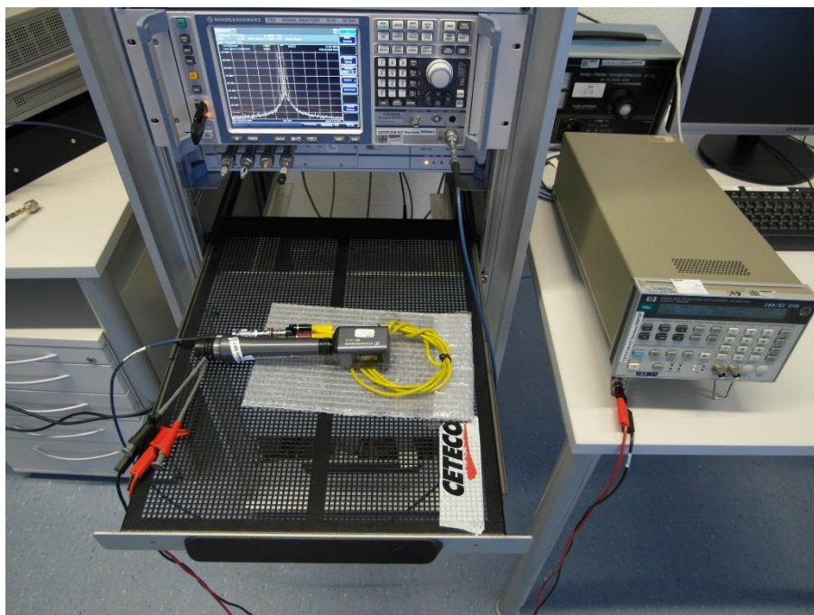
Photo 9: spectrum analyzer
