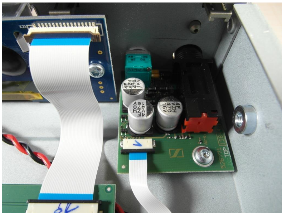
Photo 3: power supply electronic
