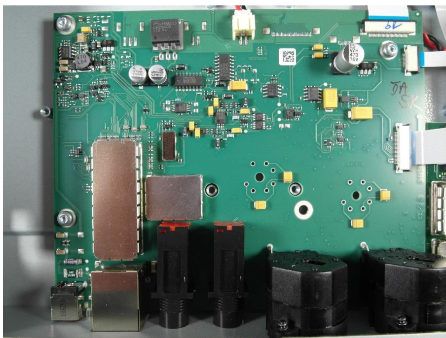
Photo 4: audio electronic with shielding
