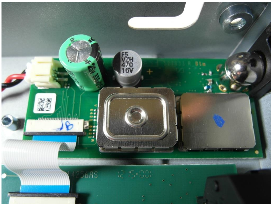
Photo 6: RF part with shielding
