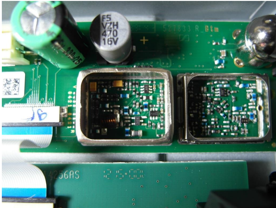
Photo 7: RF part without shielding
