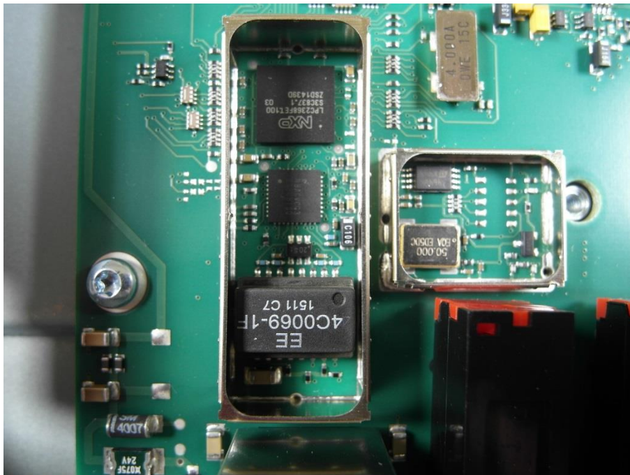
Photo 5: audio electronic without shielding
