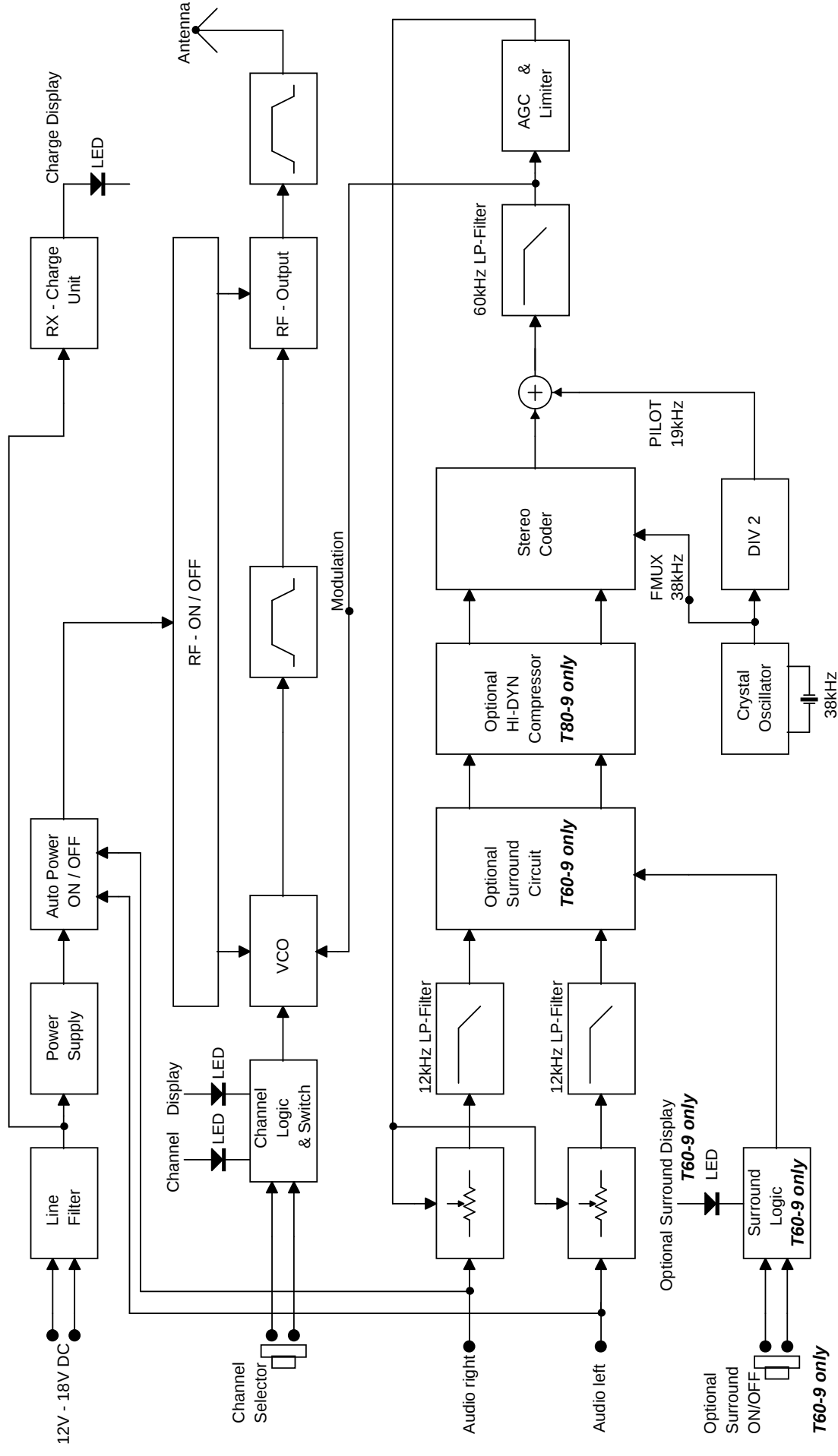
Block - Diagram TX99-9 Transmitter - Family
