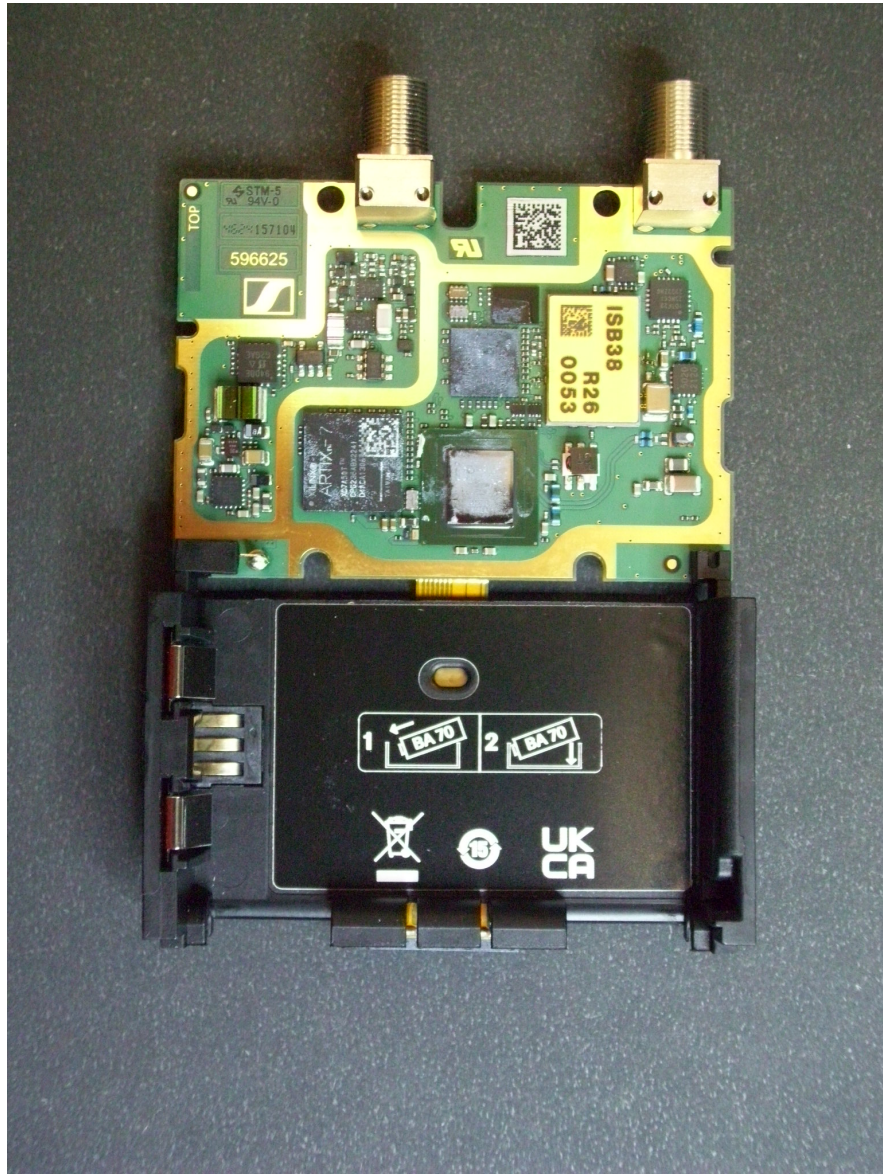
Bottom View (Main PCB)
