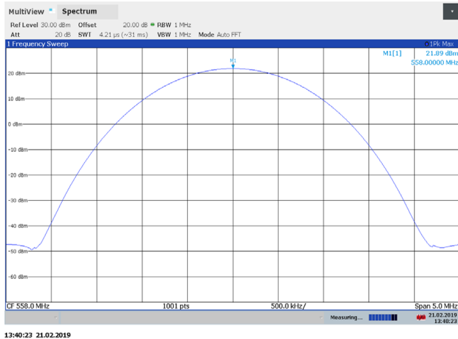
Plot 1: lowest channel, peak
