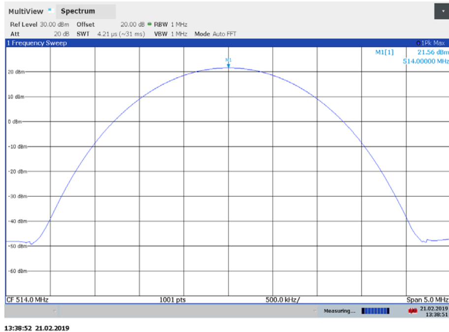
Plot 3: middle channel, peak
