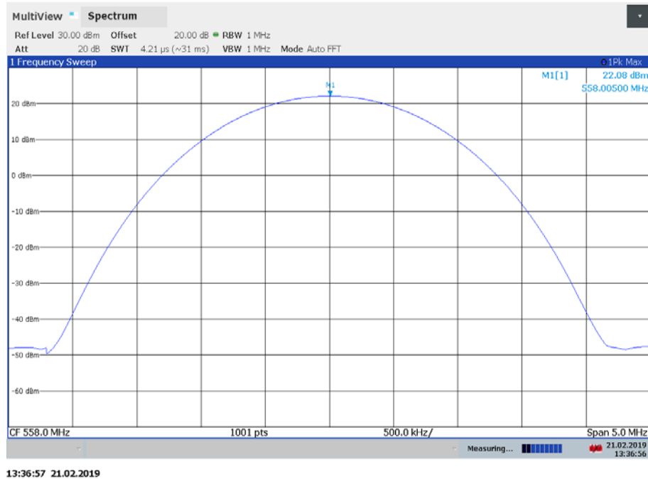
Plot 5: highest channel, peak
