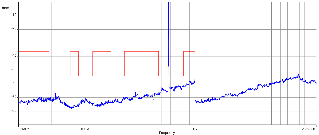
Plot 5: 579.0 MHz, spurious emissions, 25 MHz – 12.75 GHz
