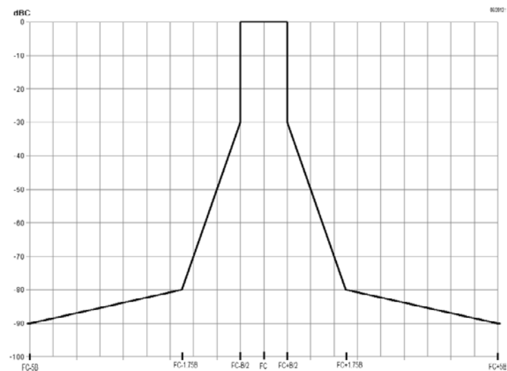
Figure .: Spectrum mask for digital systems below 2 GHz
