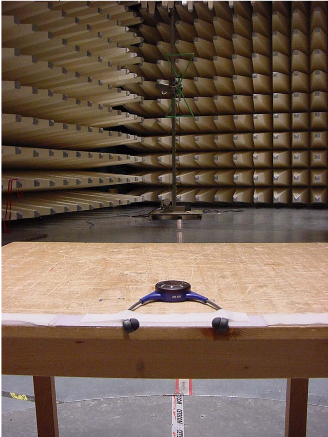
Photo 3 (Radiated Emissions): RR820
