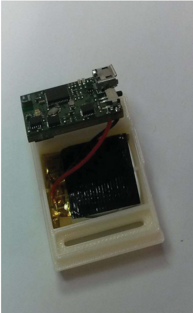
Internal PCB Top View
