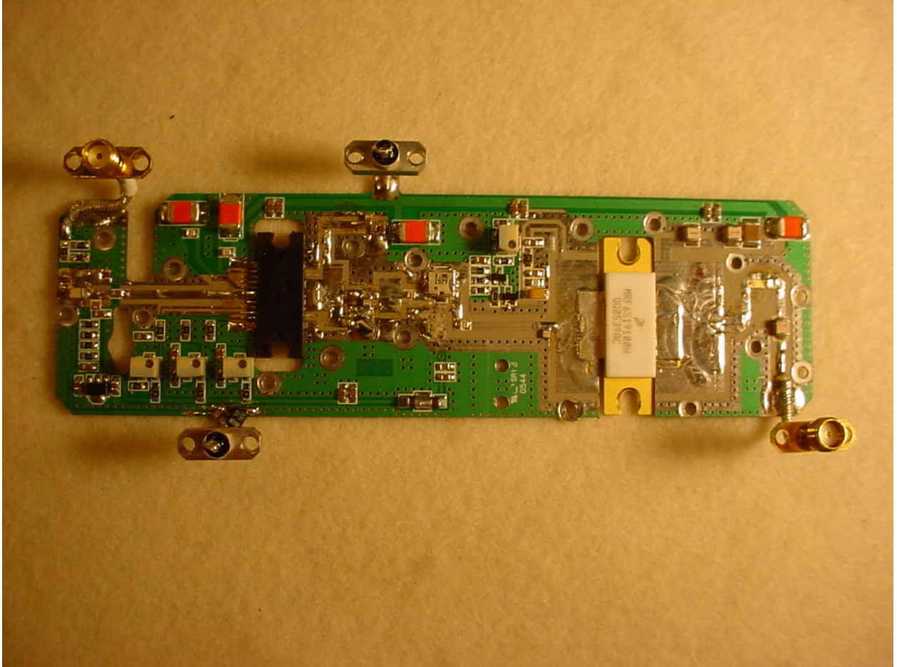
Figure 22: Internal – PA PCB Front
