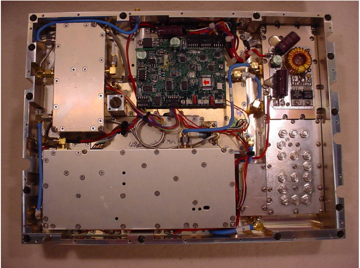
Figure 7: Internal – PA Assembled
