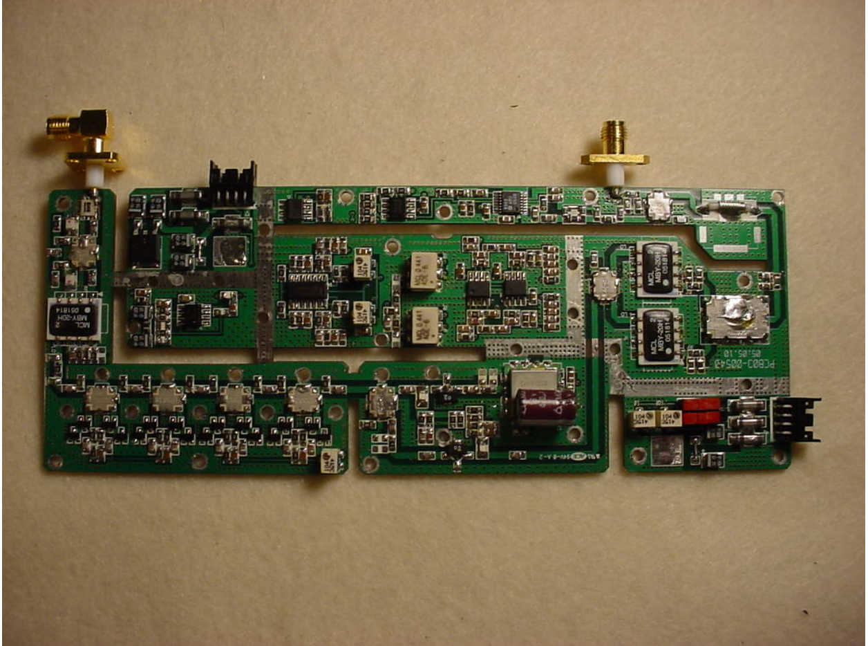
Figure 8: Internal – PA PCB Front
