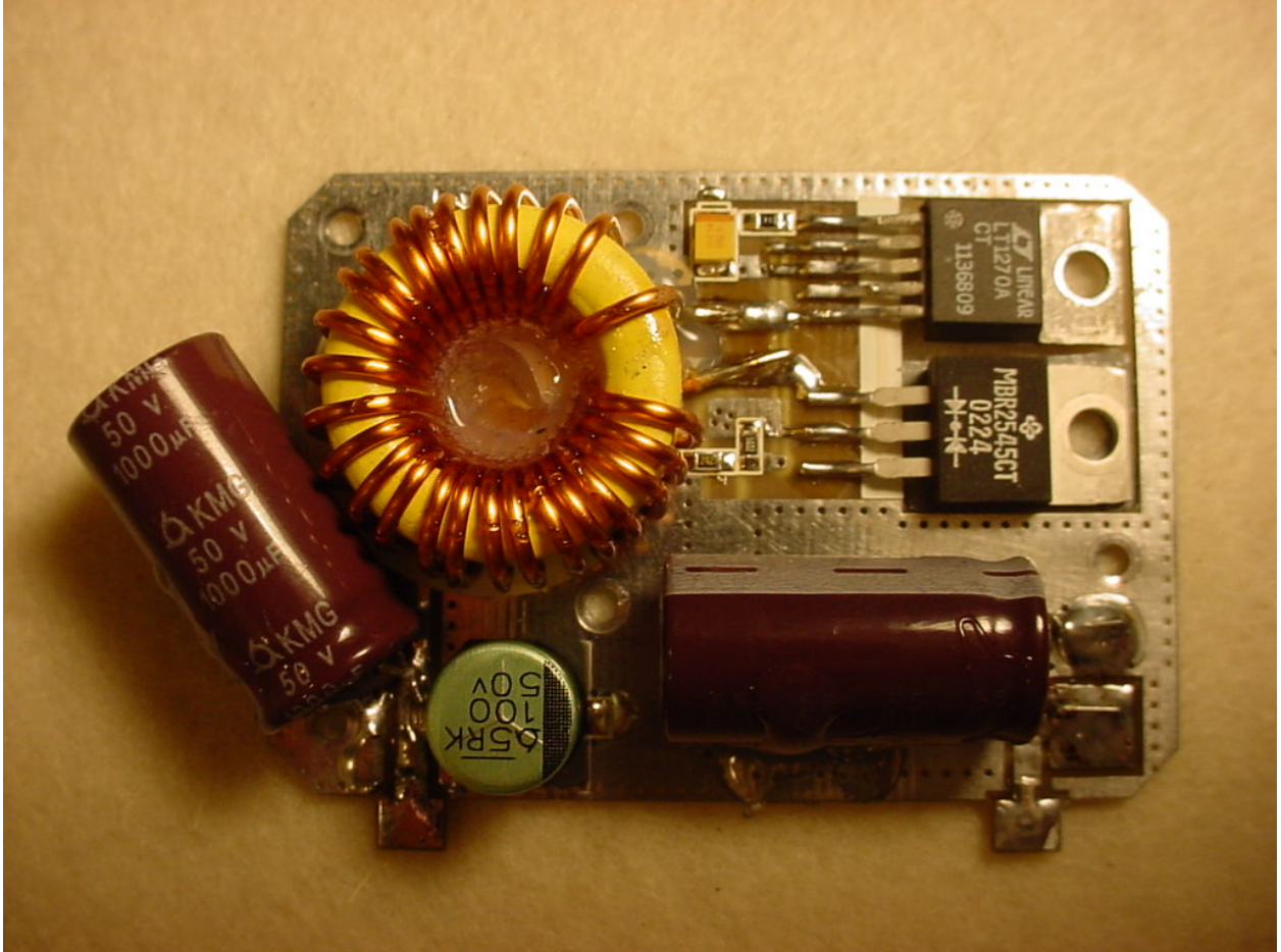
Figure 14: Internal – PA PCB Front
