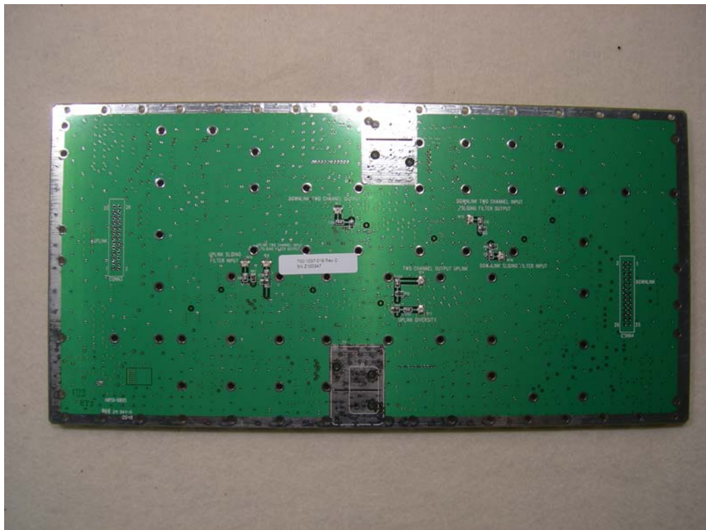
Figure 6: Internal – Channelizer RF PCB Back
