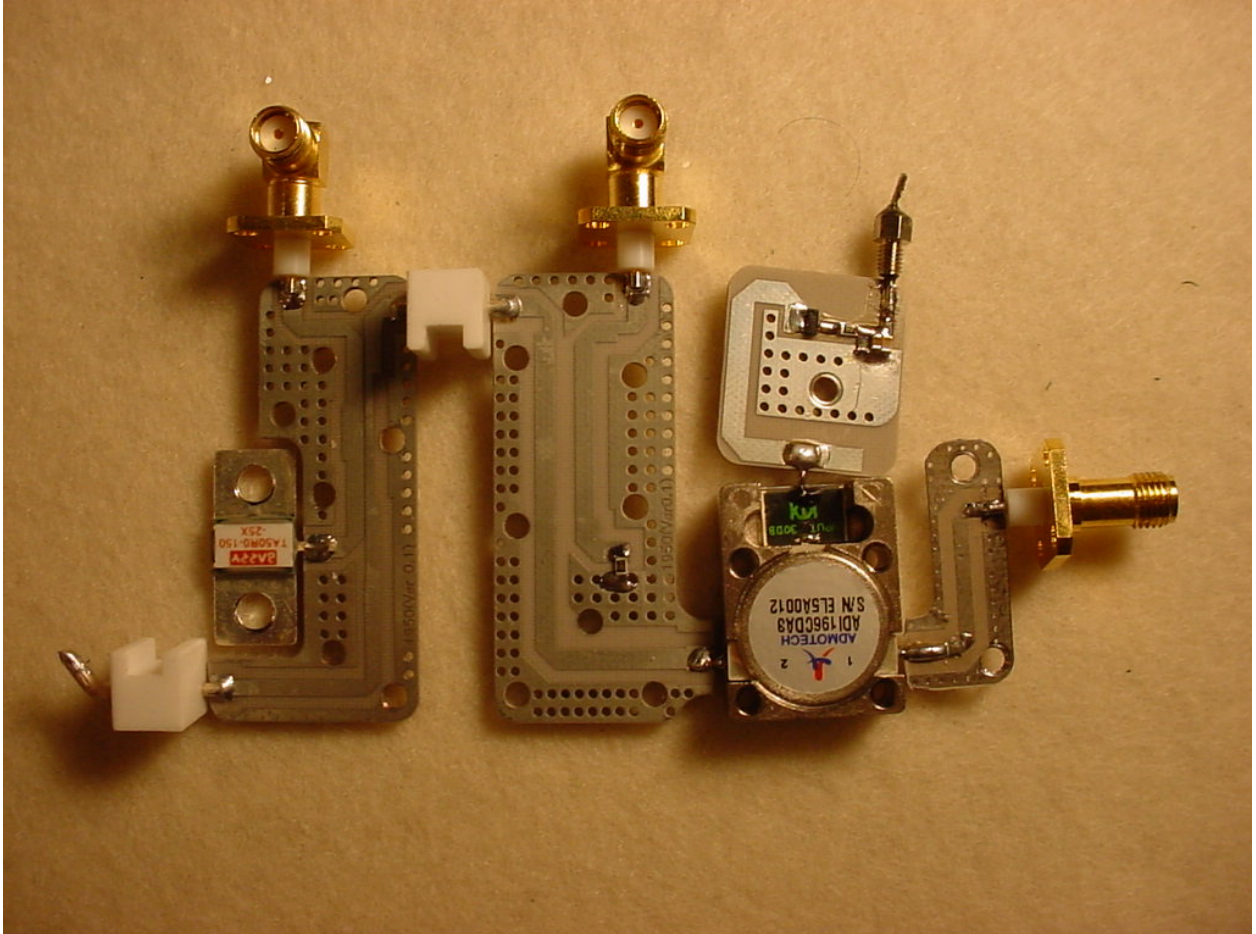
Figure 24: Internal – PA PCB Front
