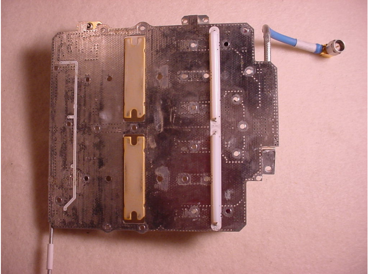
Figure 17: Internal – PA PCB Back
