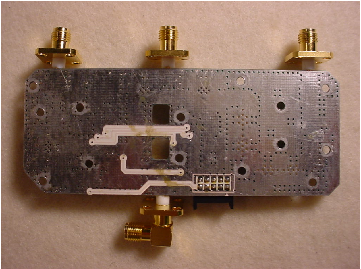
Figure 13: Internal – PA PCB Back
