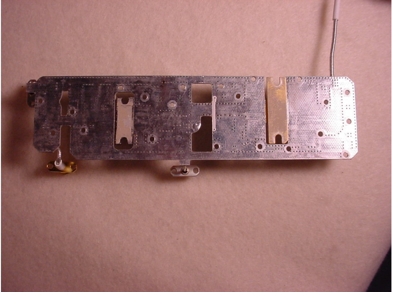
Figure 19: Internal – PA PCB Back
