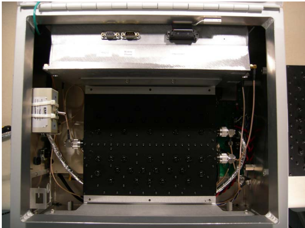
Figure 2: Internal - Assembled View – Top Duplexer Removed
