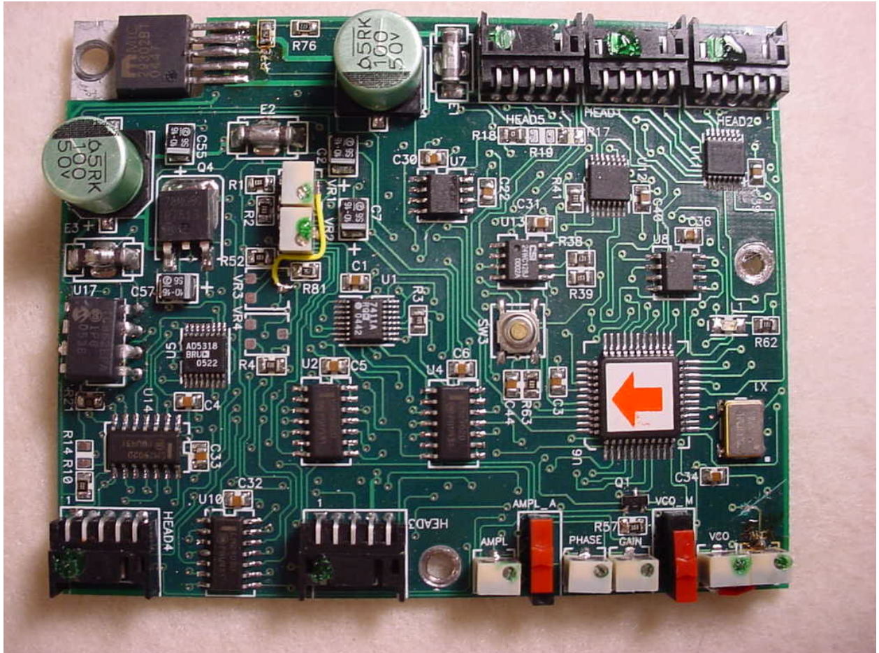
Figure 10: Internal – PA PCB Front
