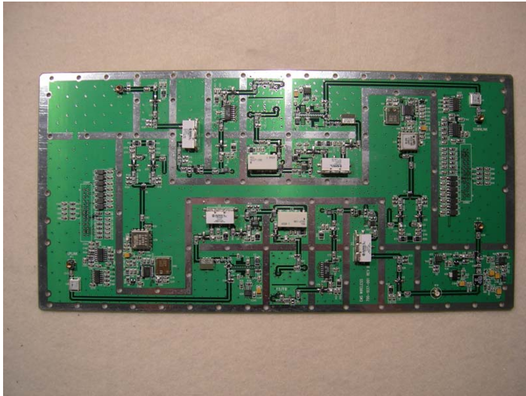
Figure 5: Internal – Channelizer RF PCB Front
