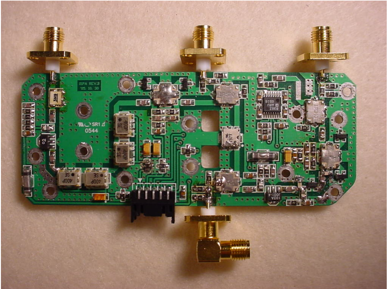
Figure 12: Internal – PA PCB Front
