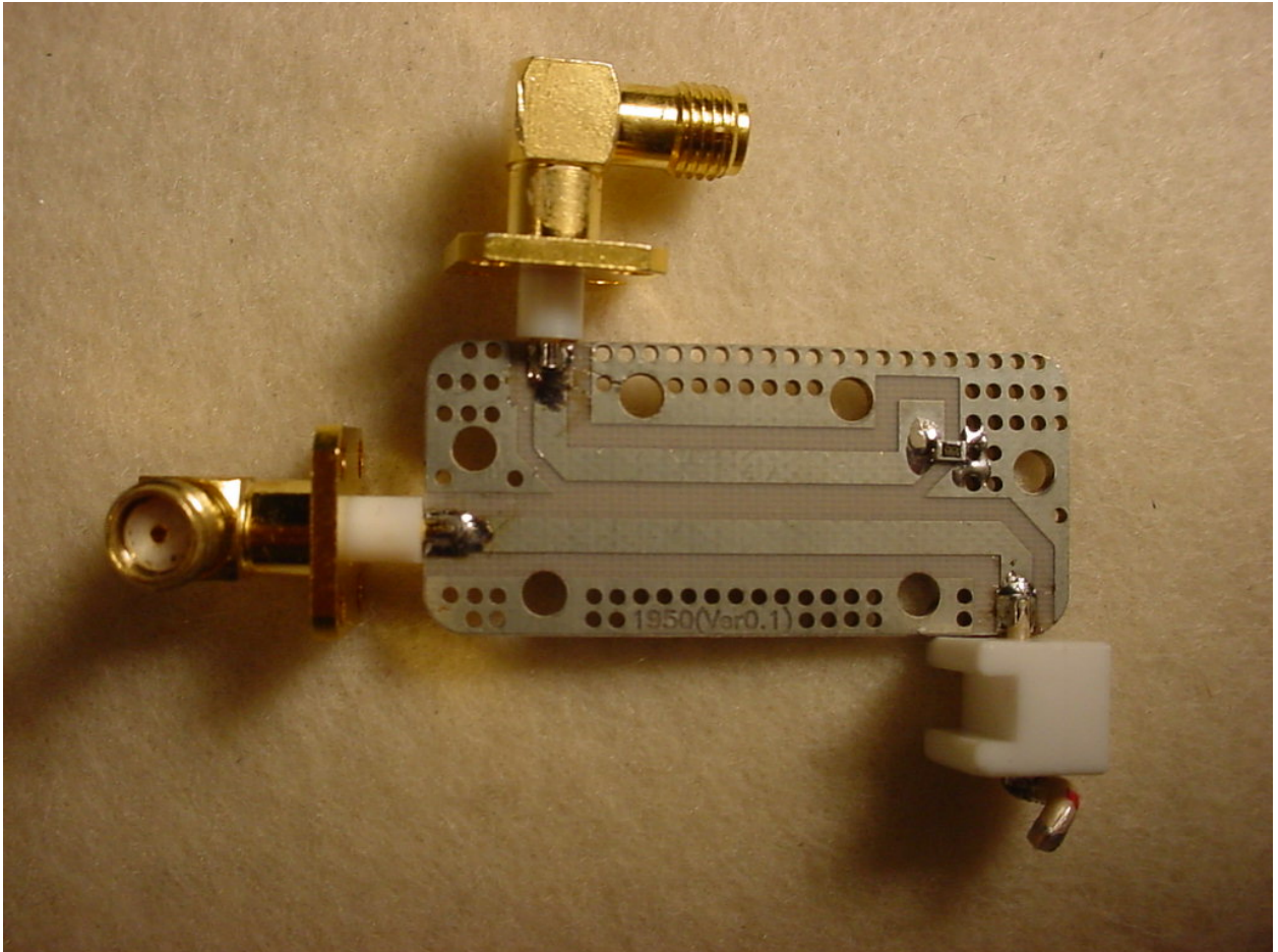
Figure 26: Internal – PA PCB Front
