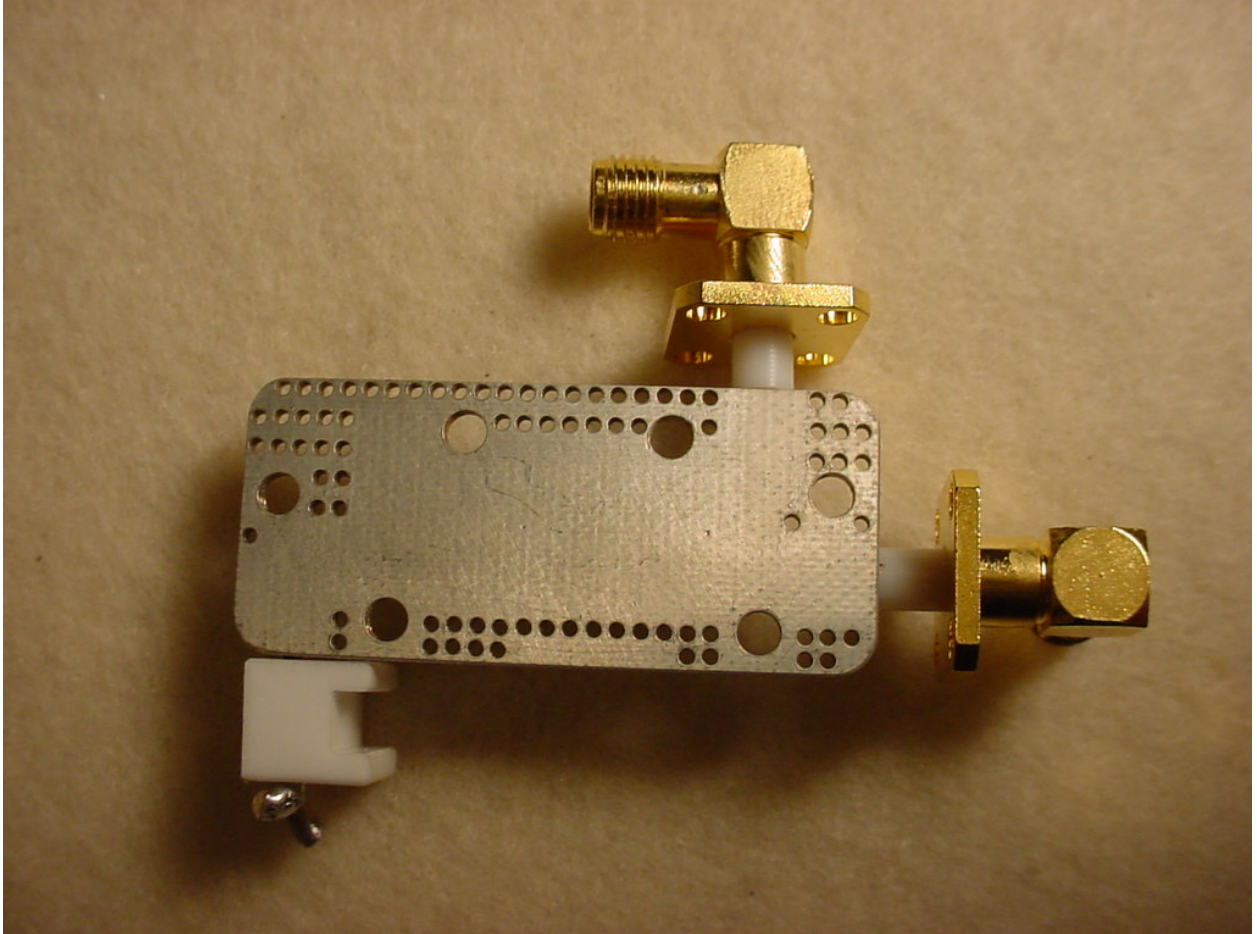
Figure 27: Internal – PA PCB Back
