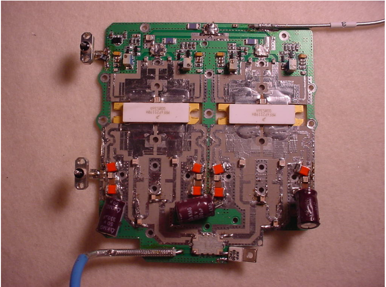
Figure 16: Internal – PA PCB Front
