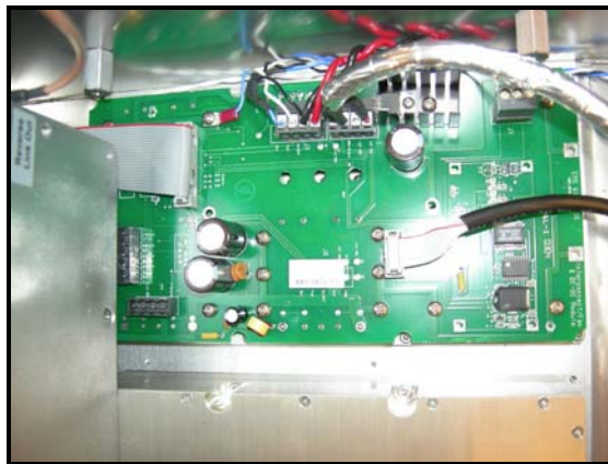
Figure 1.4-3 – Internal Photographs – Foil Wrapped Cable at DC Interconnect PCB
