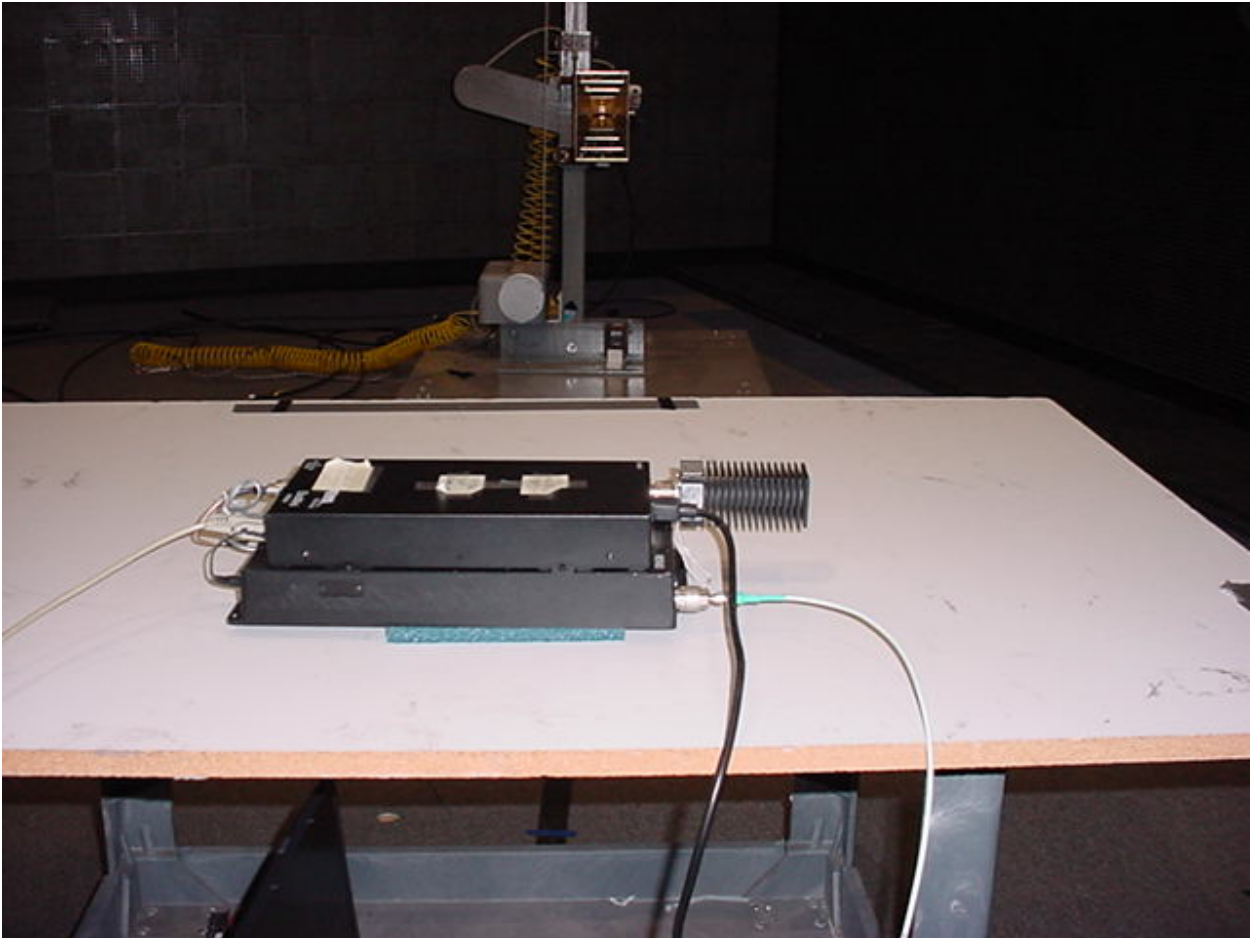
Figure 1: Test Setup – Radiated Spurious Emissions
