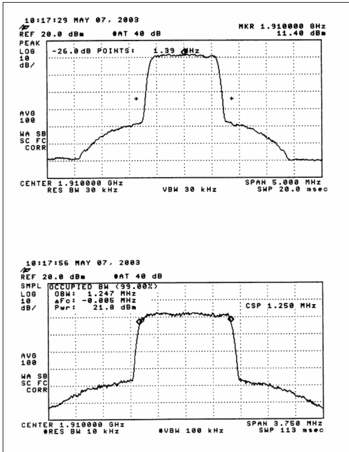
Figure 6.4.2-3: Occupied Bandwidth Plot – Uplink (High Channel)
