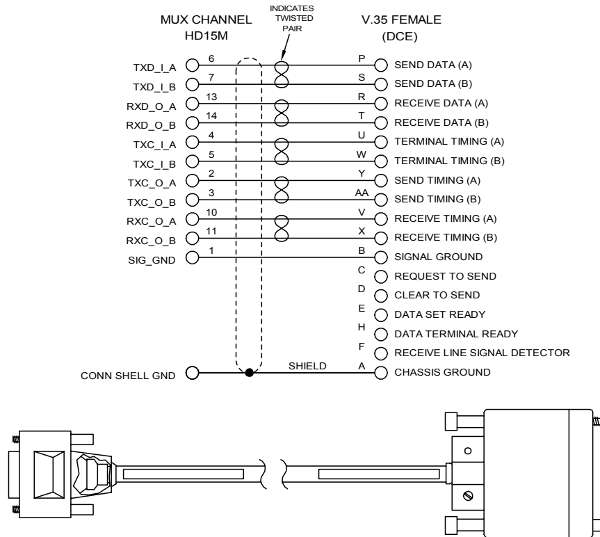
Figure 4-1. Mux Channel – V.35 (DCE)
