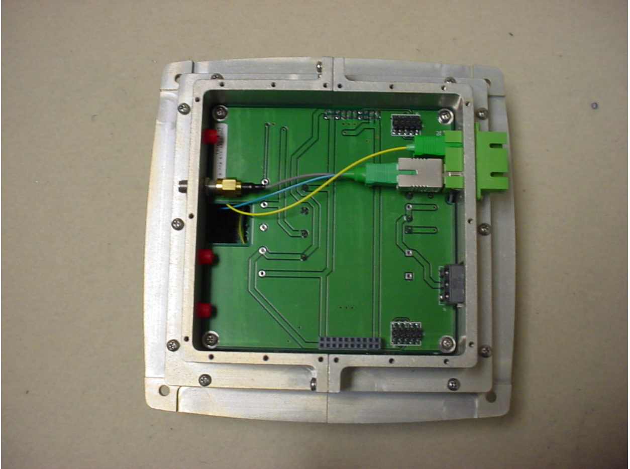
Figure 1: Internal – Assembled Top View
