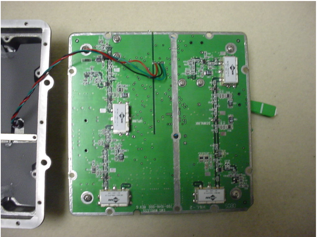
Figure 5: Internal – Micro-controller Bottom View
