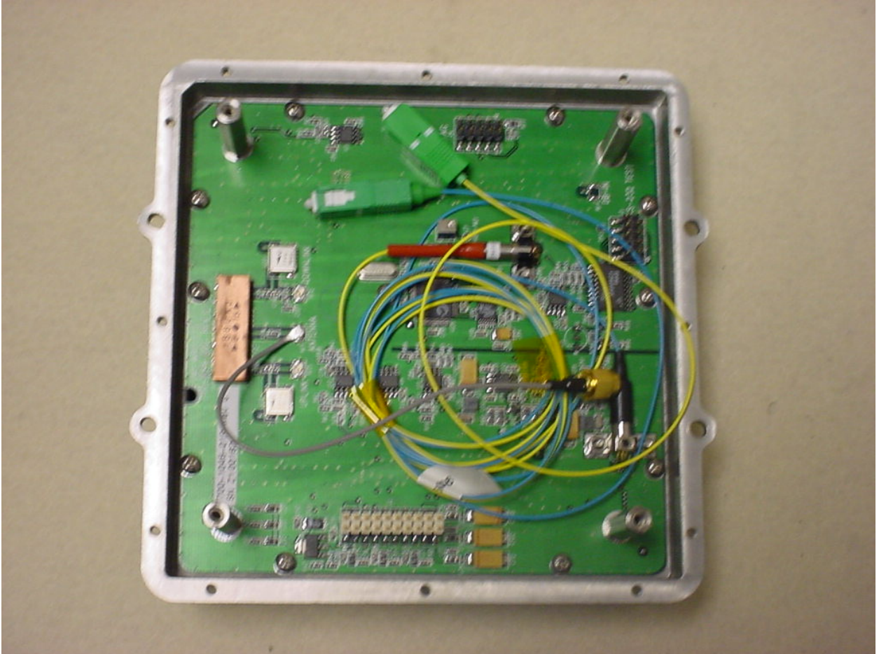
Figure 4: Internal – Micro-controller Top View
