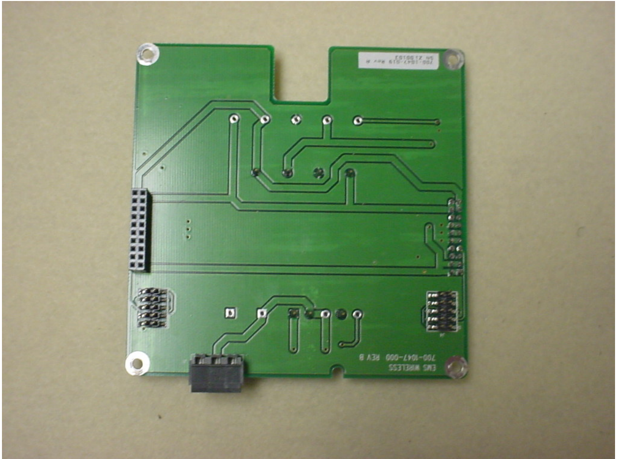
Figure 2: Internal – Power Board Top View
