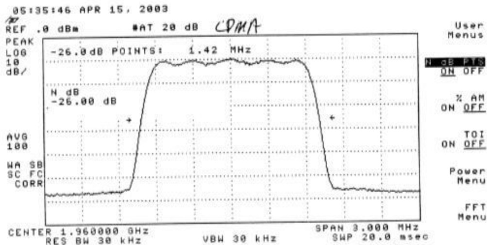
Plot 281: CDMA Mode Downlink - Middle Channel
