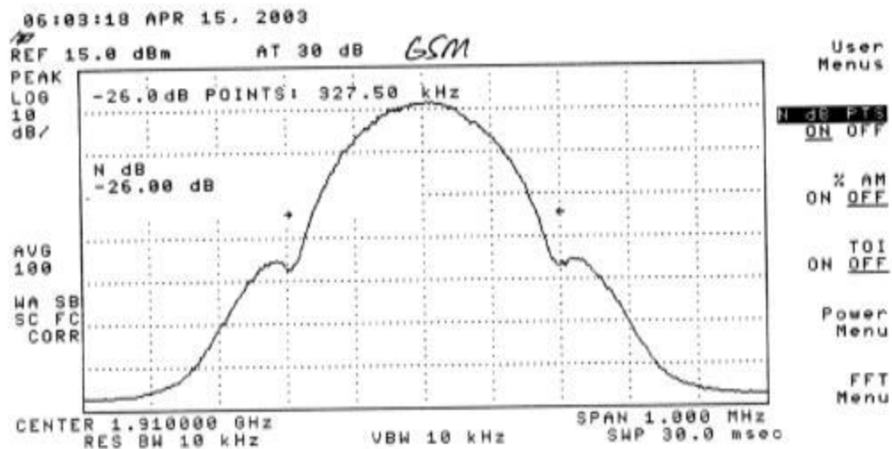
Plot 274: GSM Mode Uplink - High Channel
