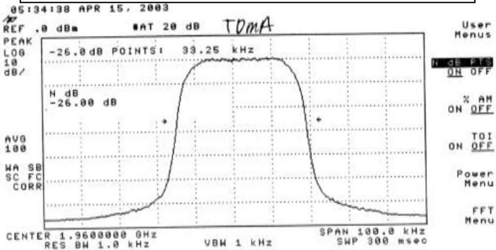
Plot 279: TDMA Mode Downlink - Middle Channel
