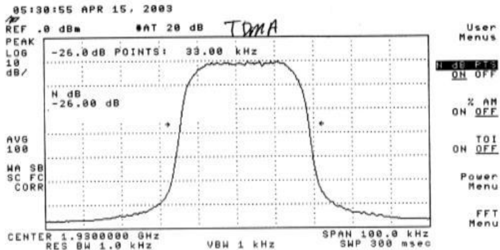
Plot 276: TDMA Mode Downlink - Low Channel
