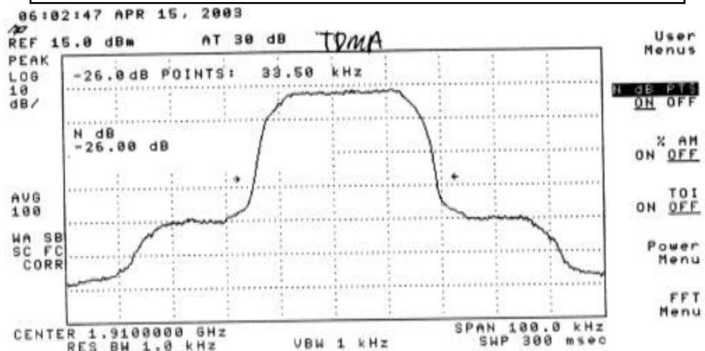
Plot 273: TDMA Mode Uplink - High Channel
