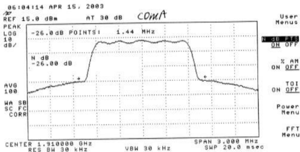
Plot 275: CDMA Mode Uplink - High Channel
