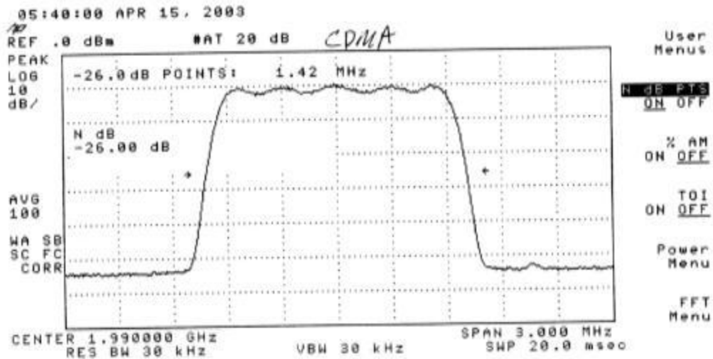
Plot 284: CDMA Mode Downlink - High Channel
