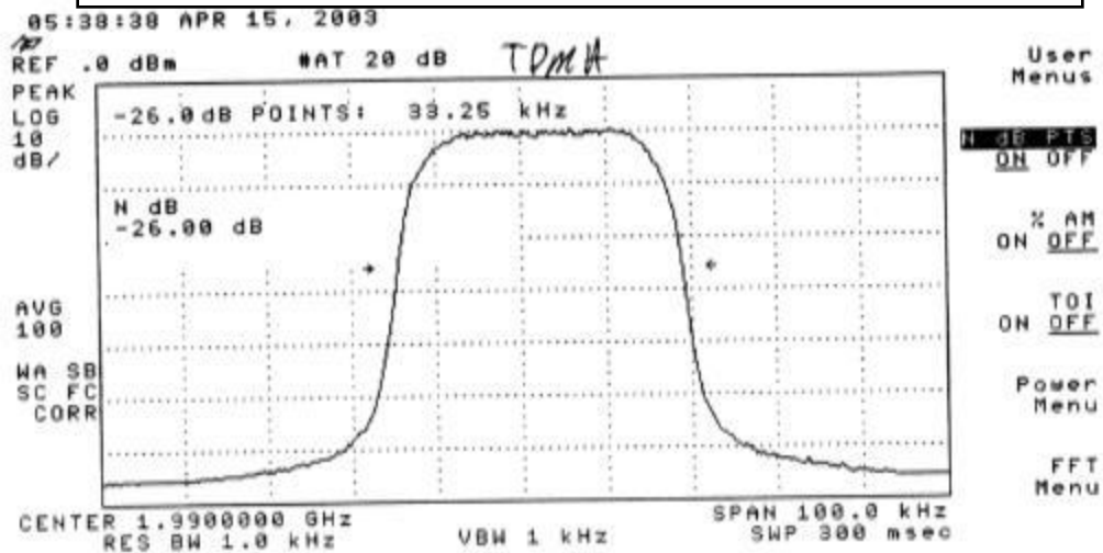
Plot 282: TDMA Mode Downlink - High Channel
