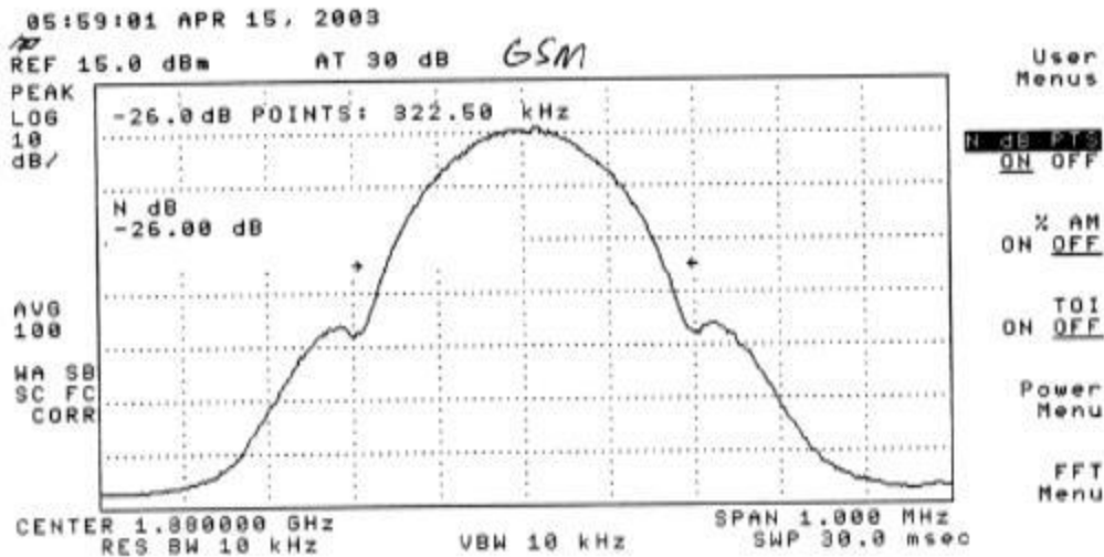
Plot 271: GSM Mode Uplink - Middle Channel
