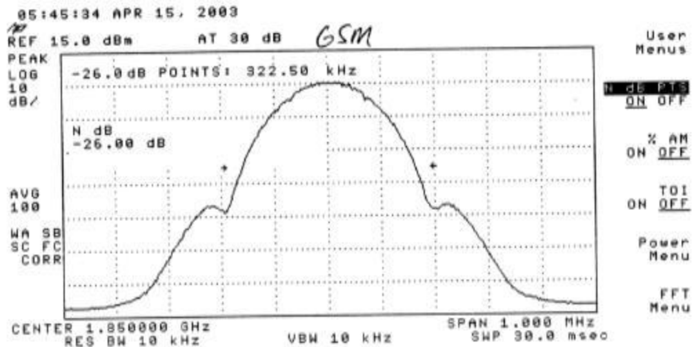
Plot 268: GSM Mode Uplink - Low Channel
