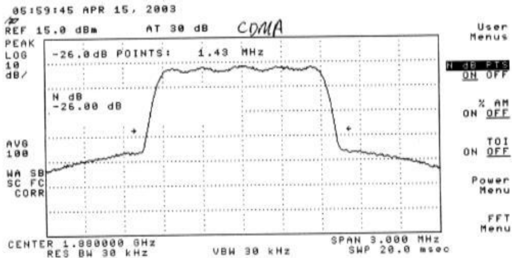
Plot 272: CDMA Mode Uplink - Middle Channel
