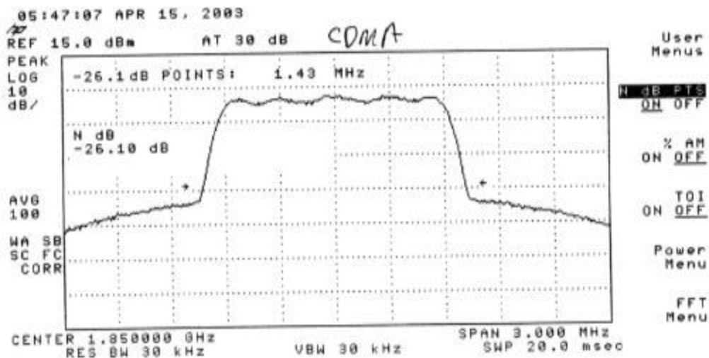
Plot 269: CDMA Mode Uplink - Low Channel
