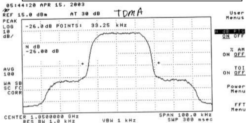
Plot 267: TDMA Mode Uplink - Low Channel
