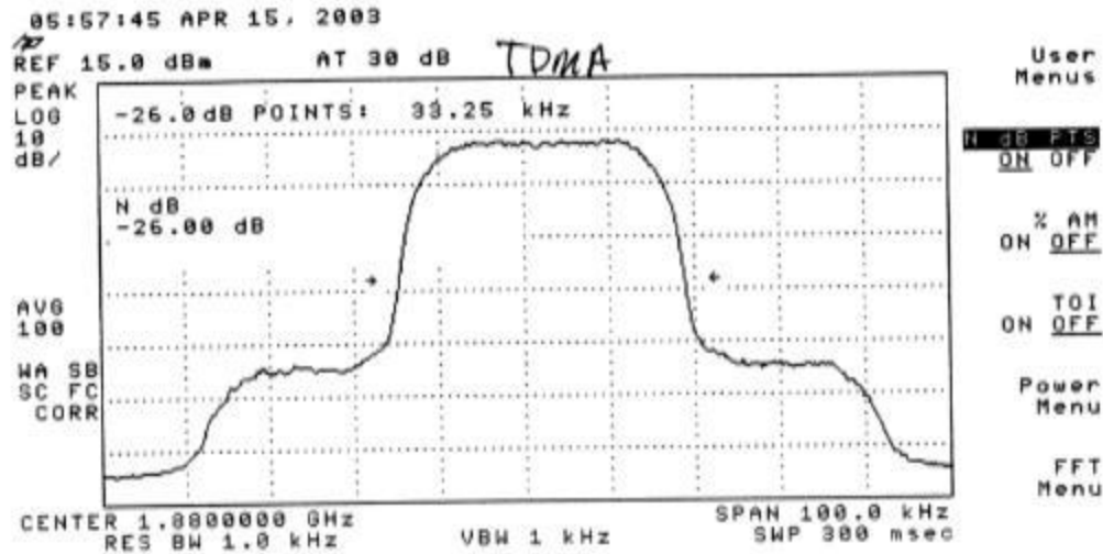
Plot 270: TDMA Mode Uplink - Middle Channel
