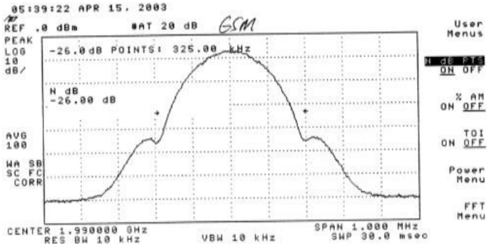
Plot 283: GSM Mode Downlink - High Channel
