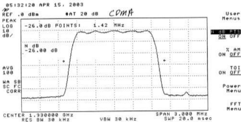
Plot 278: CDMA Mode Downlink - Low Channel
