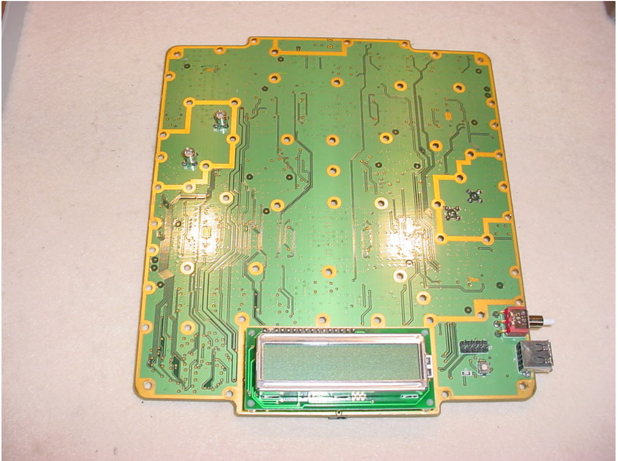
Figure 3: Internal – PCB Top View
