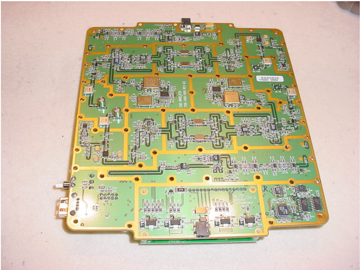
Figure 4: Internal – PCB Bottom View
