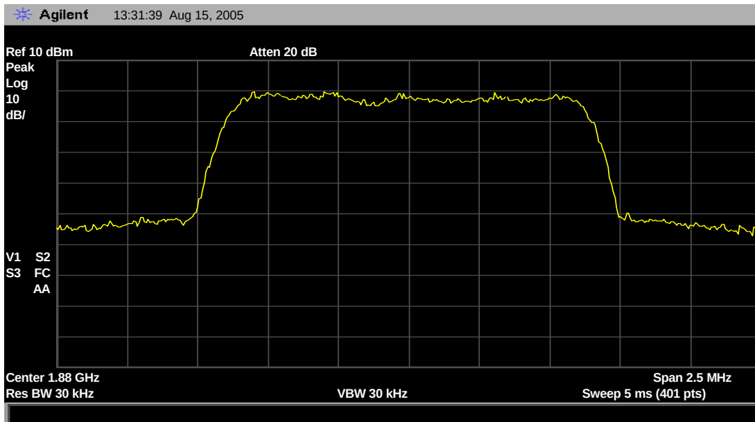
Figure 19: Occupied Bandwidth - Input Uplink CDMA Mid Channel
