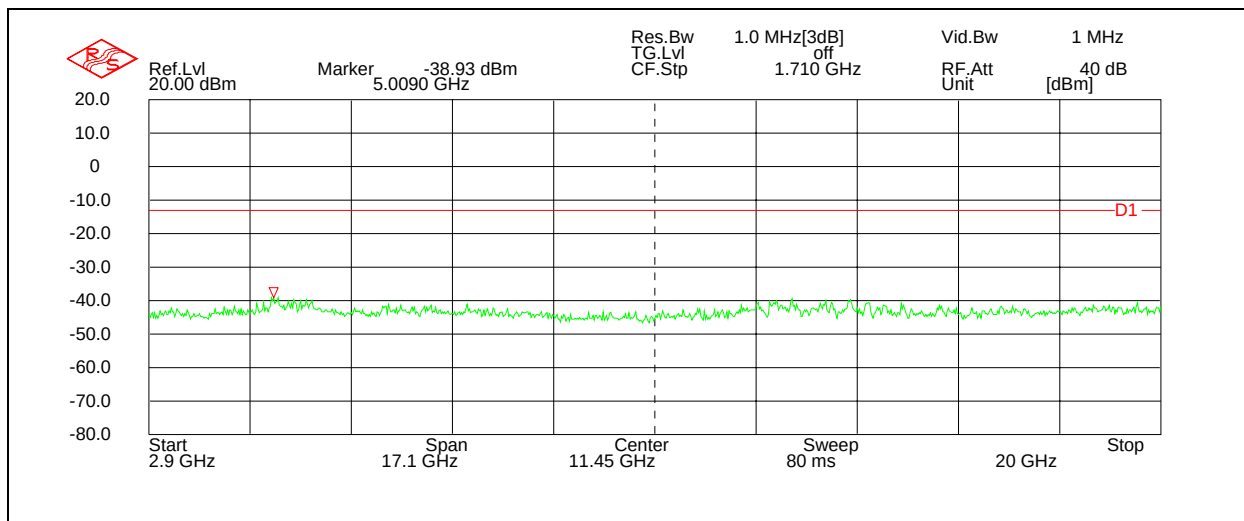
Figure 54: Spurious Emissions - Uplink GSM High Channel – 2.9 to 20 GHz
