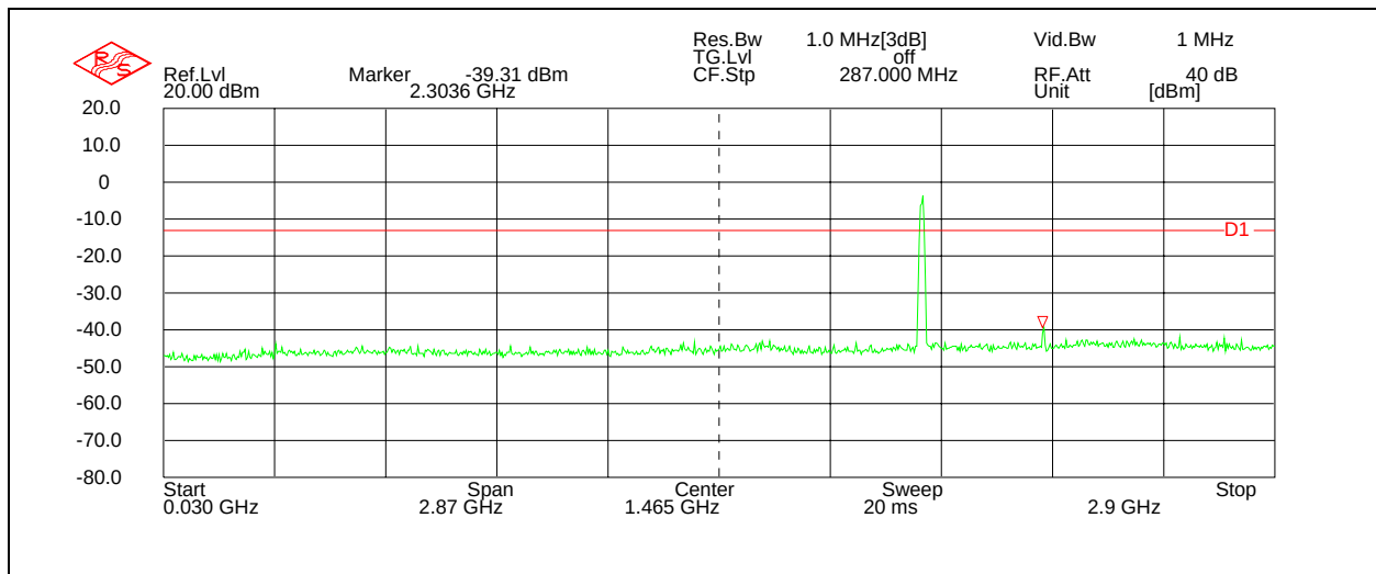
Figure 77: Spurious Emissions - Downlink GSM High Channel – 30 MHz to 2.9 GHz
