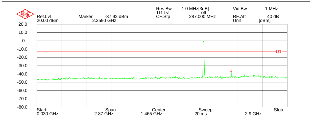
Figure 72: Spurious Emissions - Downlink GSM Low Channel – 30 MHz to 2.9 GHz
