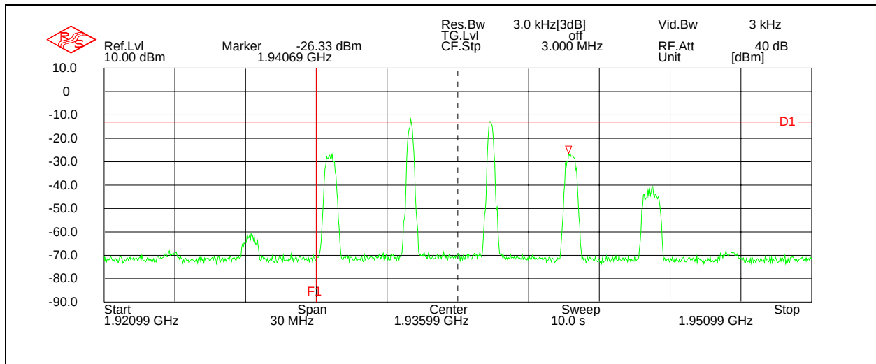
Figure 71: Spurious Emissions - Downlink GSM Low Channel – In Band
