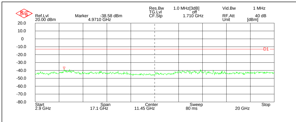
Figure 73: Spurious Emissions - Downlink GSM Low Channel – 2.9 to 20 GHz
