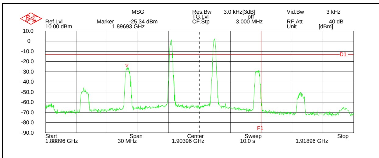
Figure 52: Spurious Emissions - Uplink GSM High Channel – In Band
