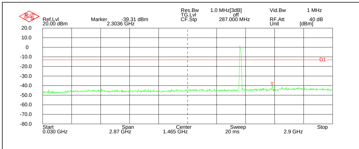
Figure 61: Spurious Emissions - Downlink CDMA High Channel – 30 MHz to 2.9 GHz
