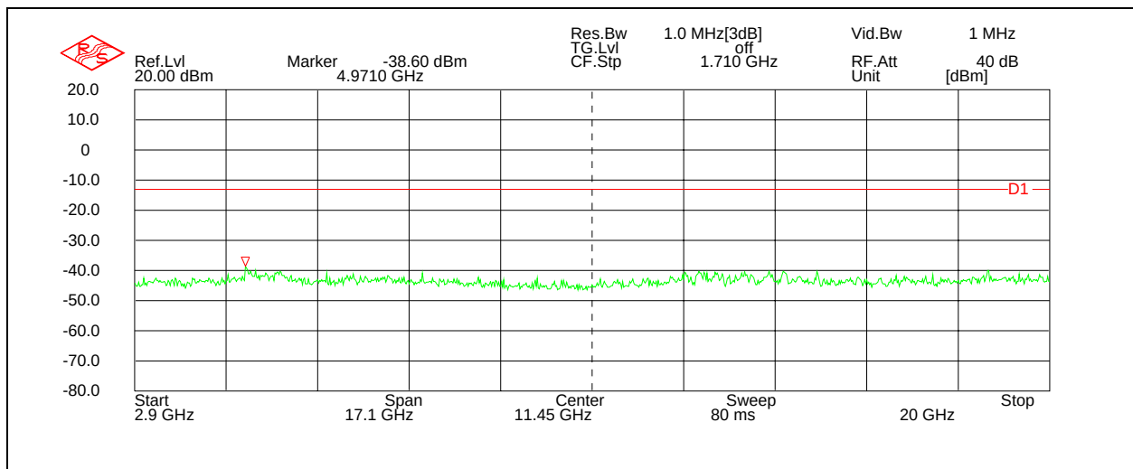
Figure 38: Spurious Emissions - Uplink CDMA High Channel – 2.9 to 20 GHz
