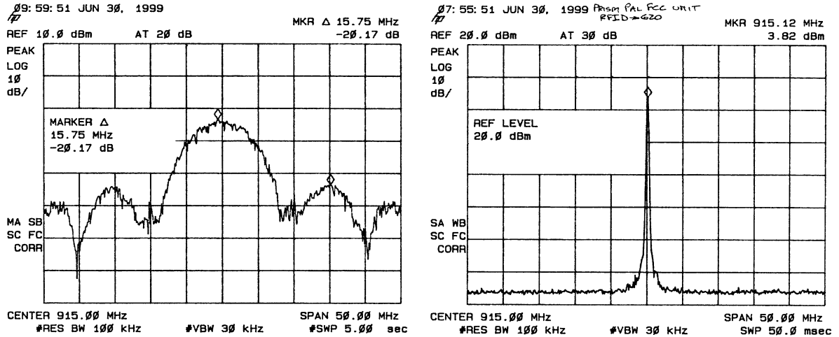
Figure 3: PAL Modulation Spectra & Peak Power Output
