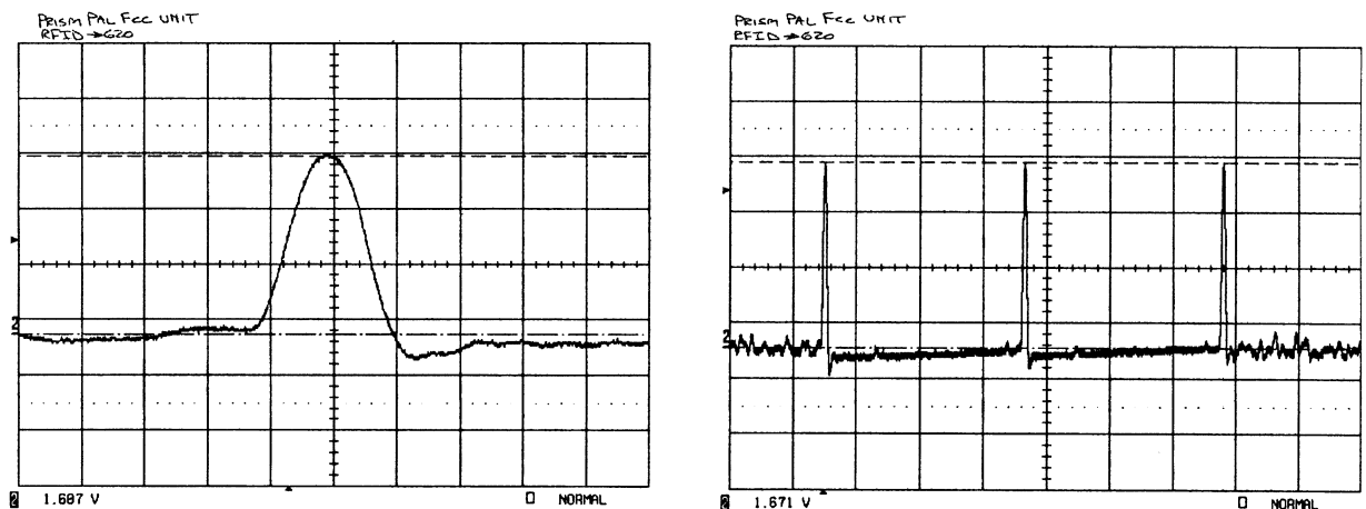
Figure 6: Correlation Pulse from PAL Transmitter
