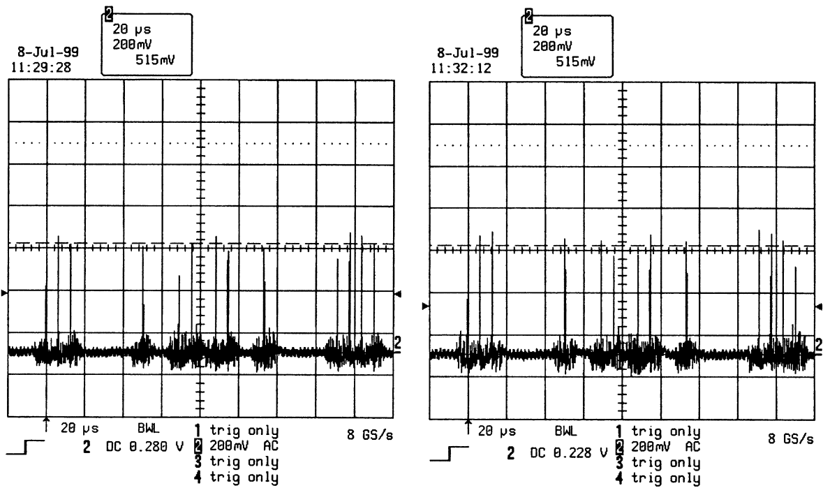
Figure 10: Correlator Output Pulses V_2 ; Amplitude with CW Interferor Signal
