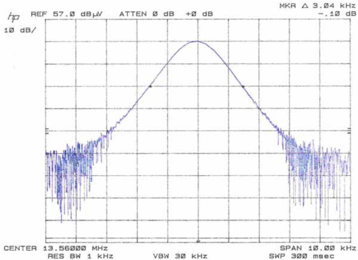
Figure 1. Occupied Bandwidth
