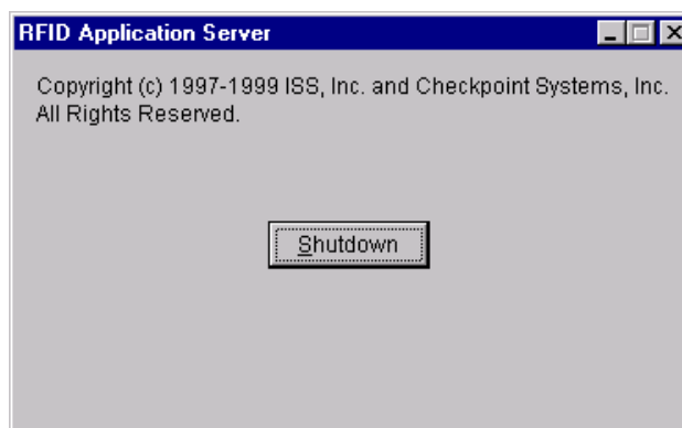
Figure 4-36: Shutdown Button
