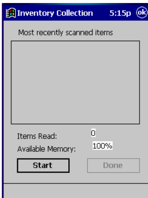
Figure 3-11: Inventory Collection
