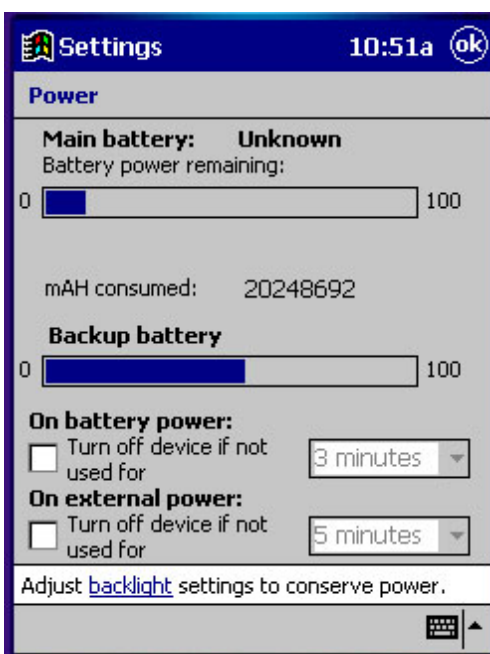
Figure 3-7: Battery Status
