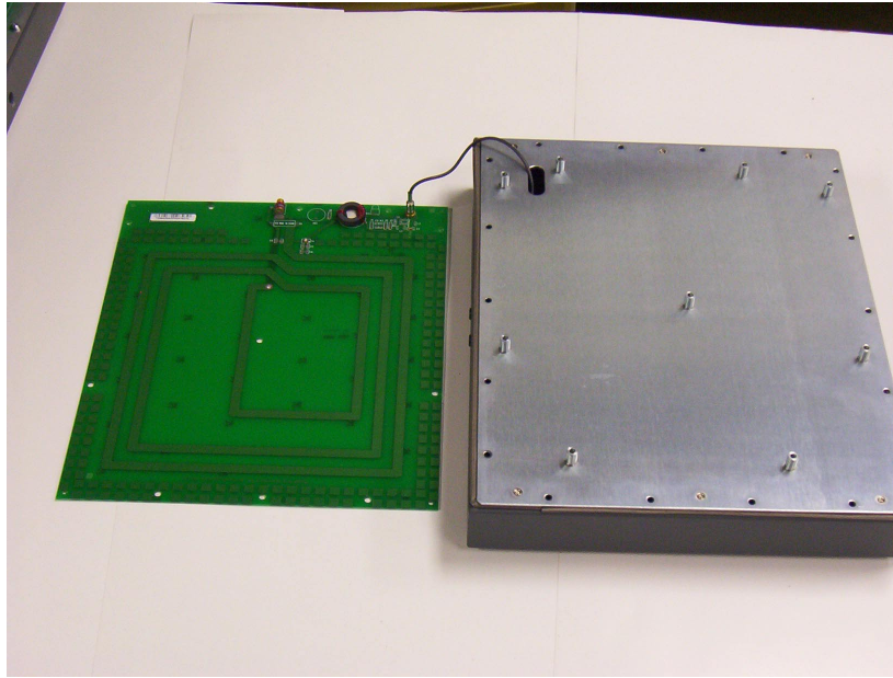
Top cover removed, antenna PCB removed
