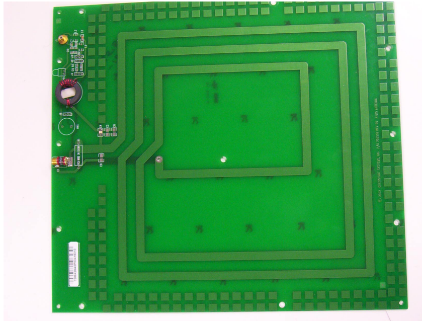
Antenna PCB top
