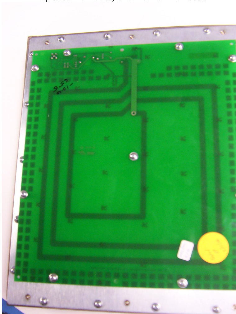
Antenna Assembly
