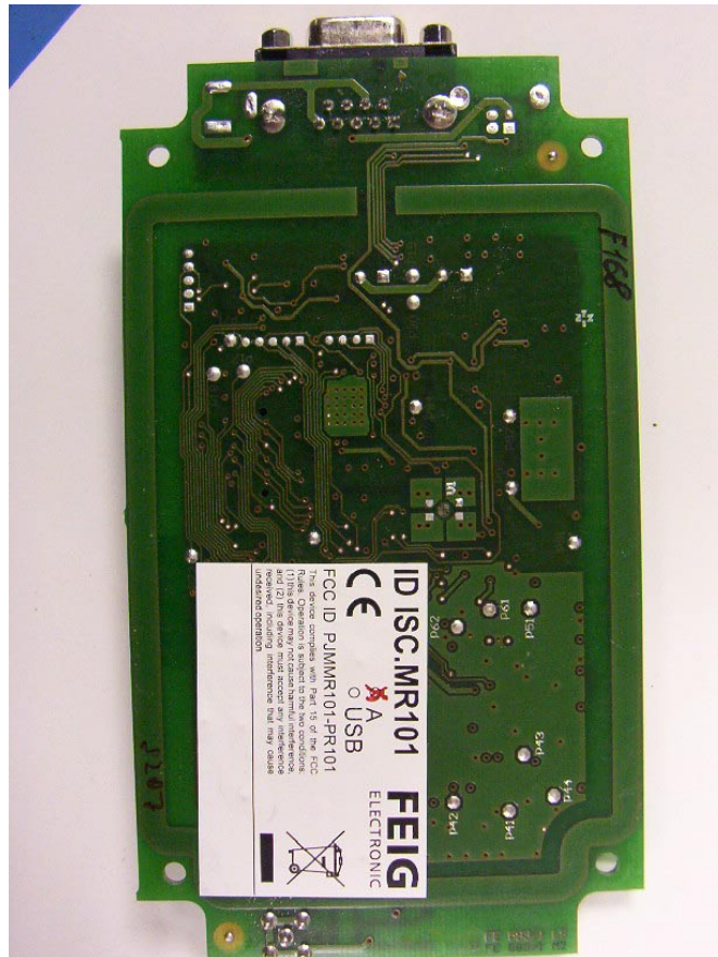
Transmitter PCB bottom
