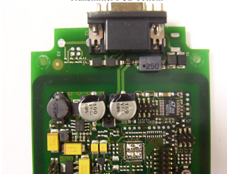
Transmitter PCB Top 1
