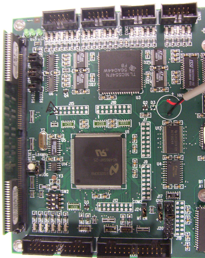
Single Board Computer PCB top 1
