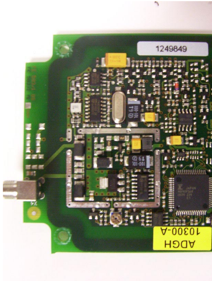
Transmitter PCB Top 2
