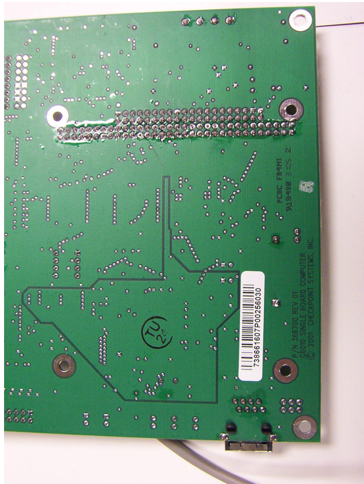
Single Board Computer PCB bottom 1
