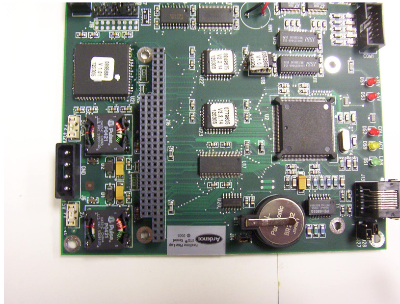
Single Board Computer PCB top 1
