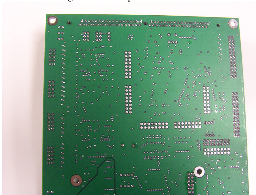
Single Board Computer PCB bottom 2
