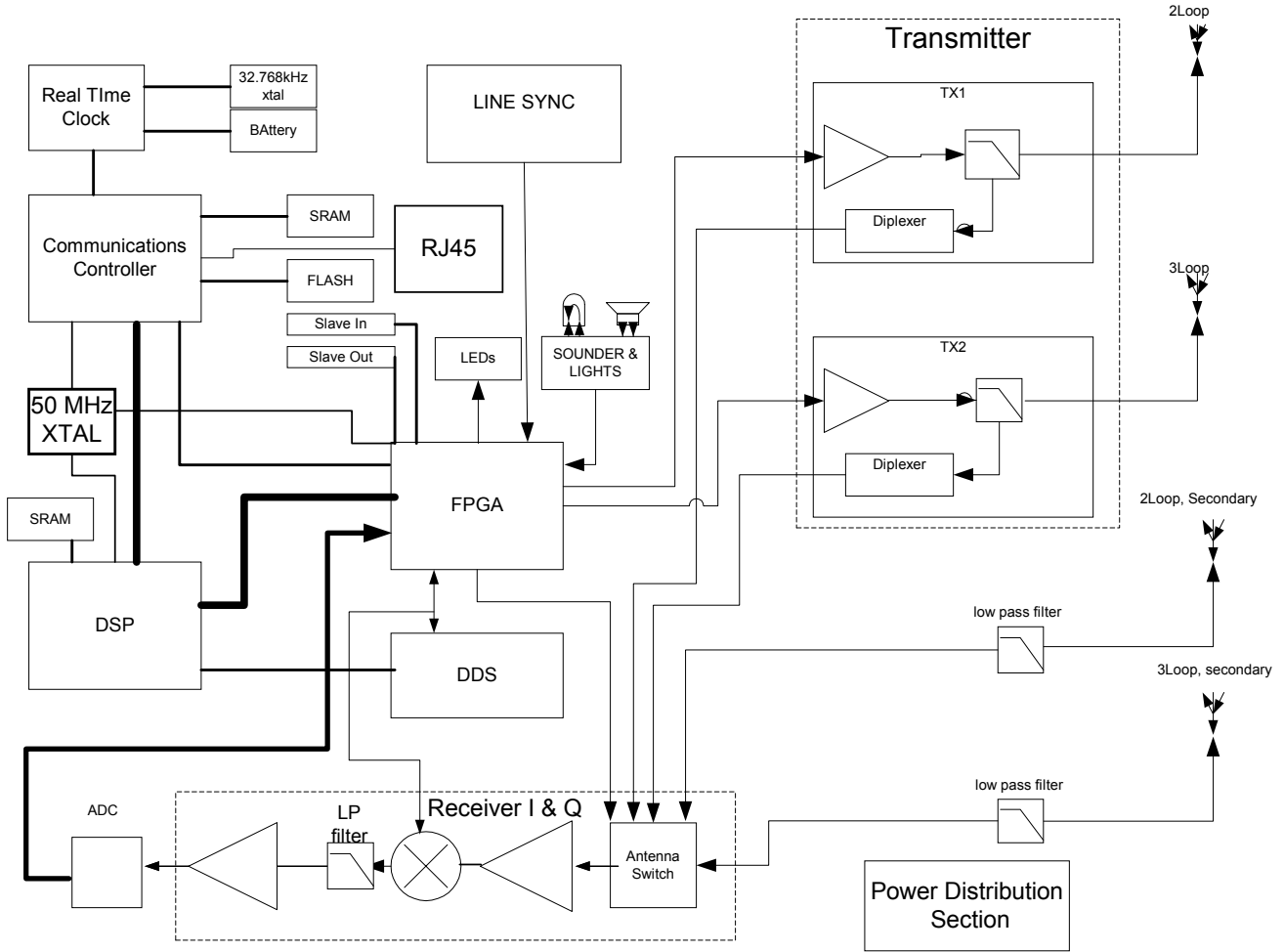
Figure 1. Overall Block Diagram for the TR4024
